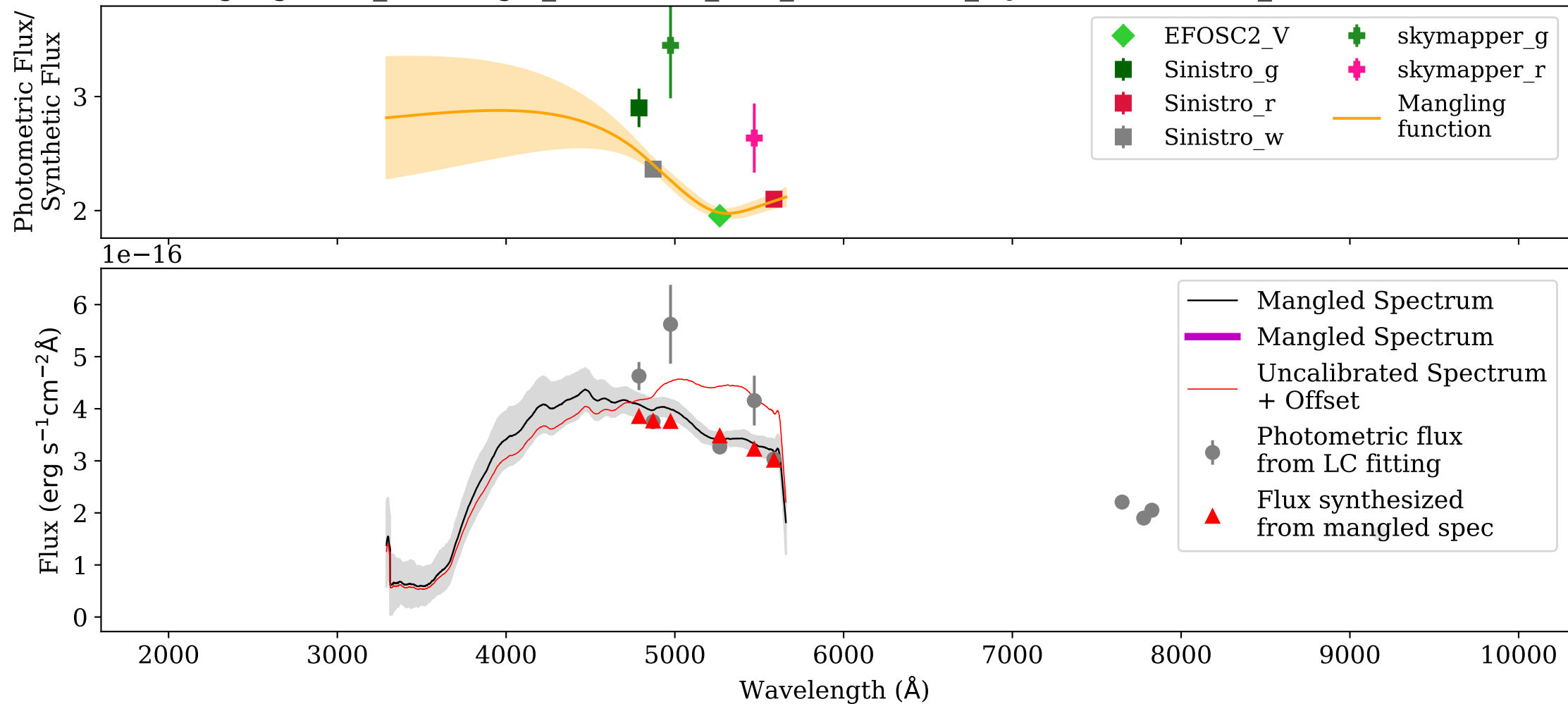
Mangling: UVB_AT2017gfo_ENGRAVE_v1.0_XSHOOTER_MJD-57983.969002_Phase+1.43d.dat
