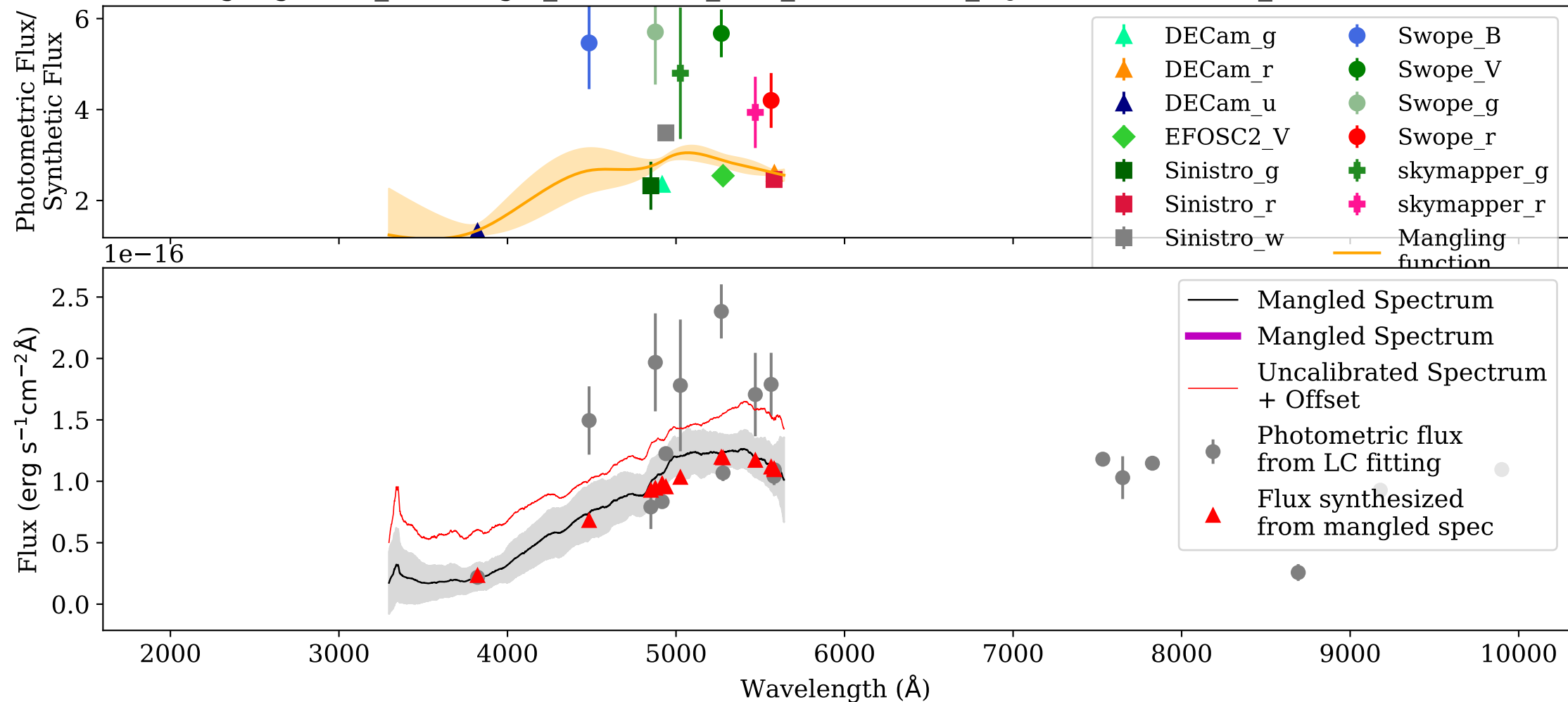
Mangling: UVB_AT2017gfo_ENGRAVE_v1.0_XSHOOTER_MJD-57984.969002_Phase+2.42d.dat
