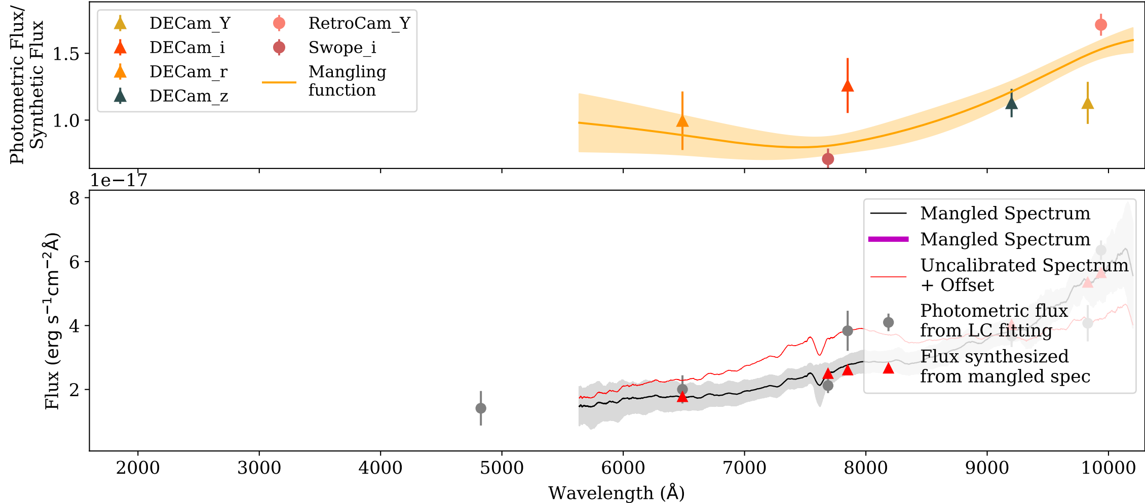
Mangling: VIS_AT2017gfo_ENGRAVE_v1.0_XSHOOTER_MJD-57987.980003_Phase+5.40d.dat
