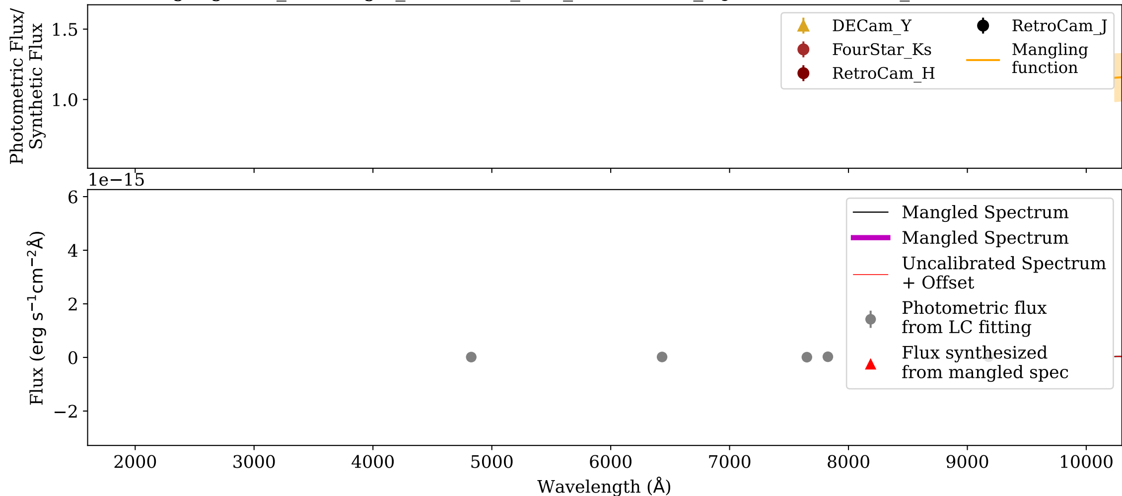
Mangling: NIR_AT2017gfo_ENGRAVE_v1.0_XSHOOTER_MJD-57988.990001_Phase+6.40d.dat
