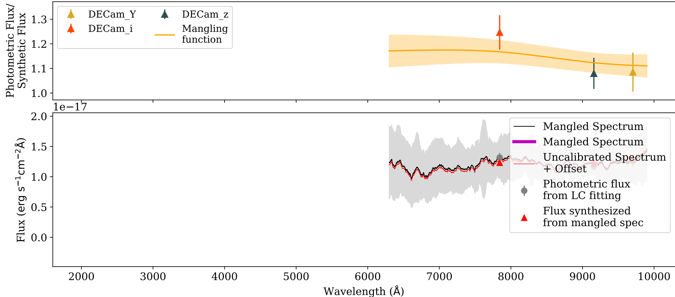
Mangling: VIS_AT2017gfo_ENGRAVE_v1.0_XSHOOTER_MJD-57991.000003_Phase+8.40d.dat
