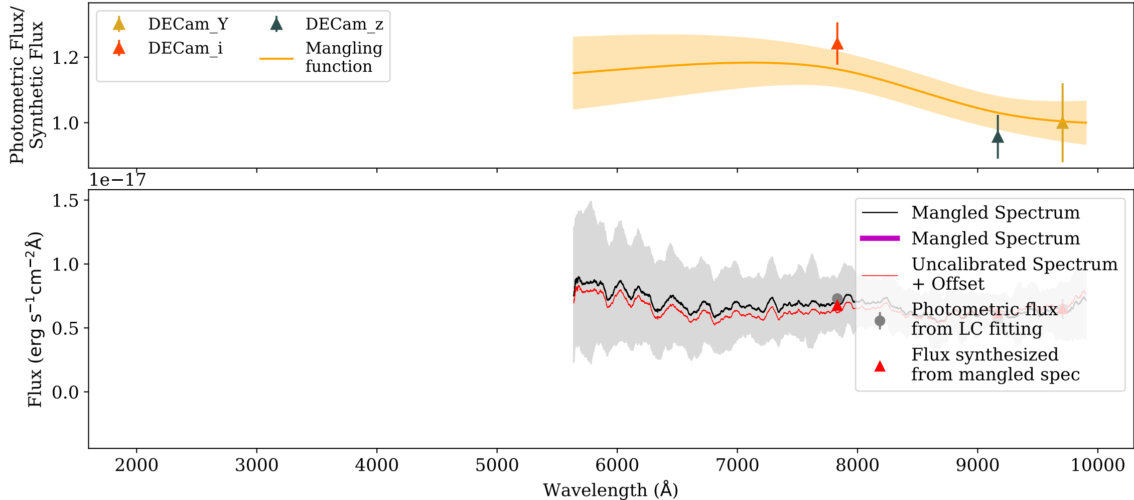
Mangling: VIS_AT2017gfo_ENGRAVE_v1.0_XSHOOTER_MJD-57992.000003_Phase+9.40d.dat
