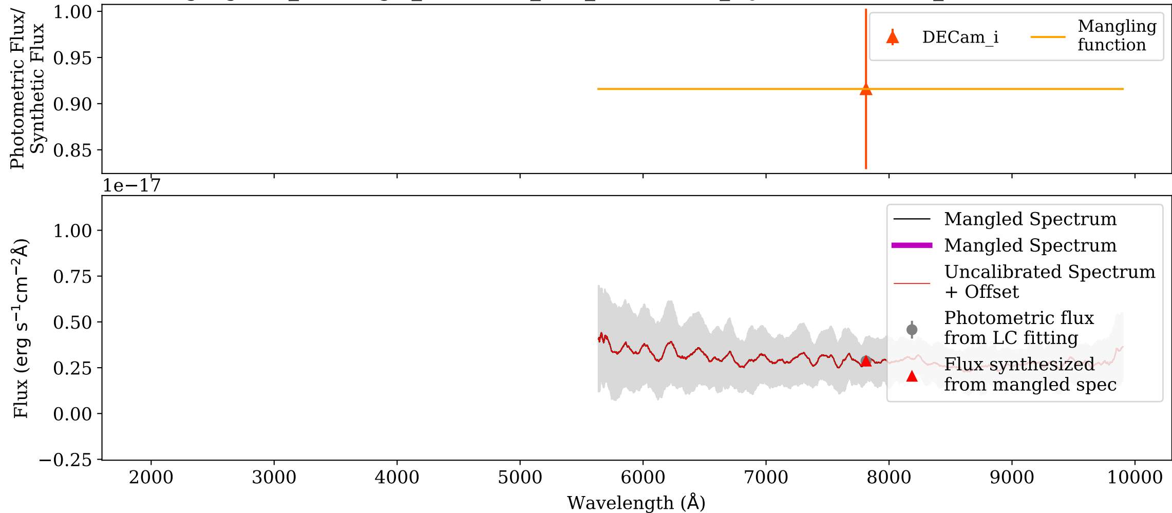
Mangling: VIS_AT2017gfo_ENGRAVE_v1.0_XSHOOTER_MJD-57993.000003_Phase+10.40d.dat
