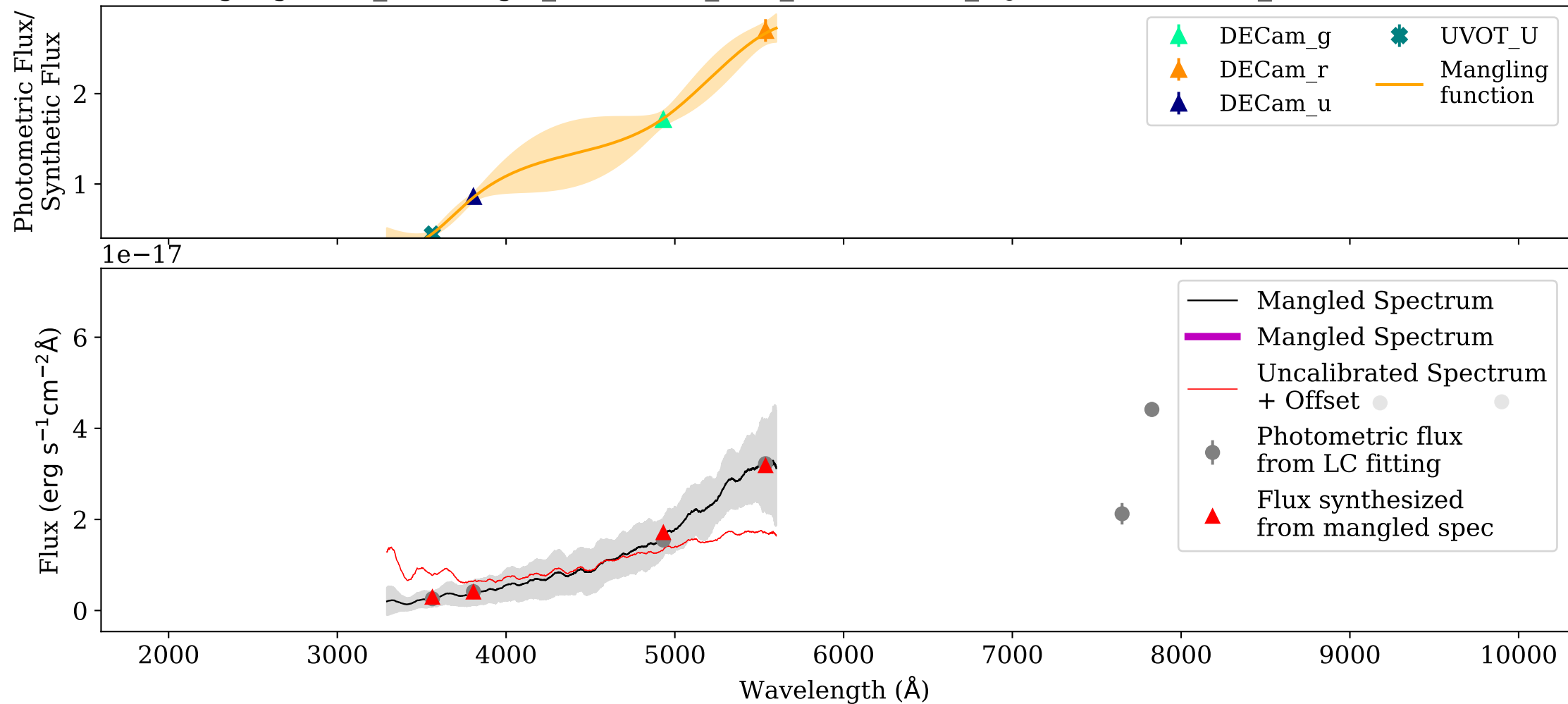
Mangling: UVB_AT2017gfo_ENGRAVE_v1.0_XSHOOTER_MJD-57987.980002_Phase+5.40d.dat
