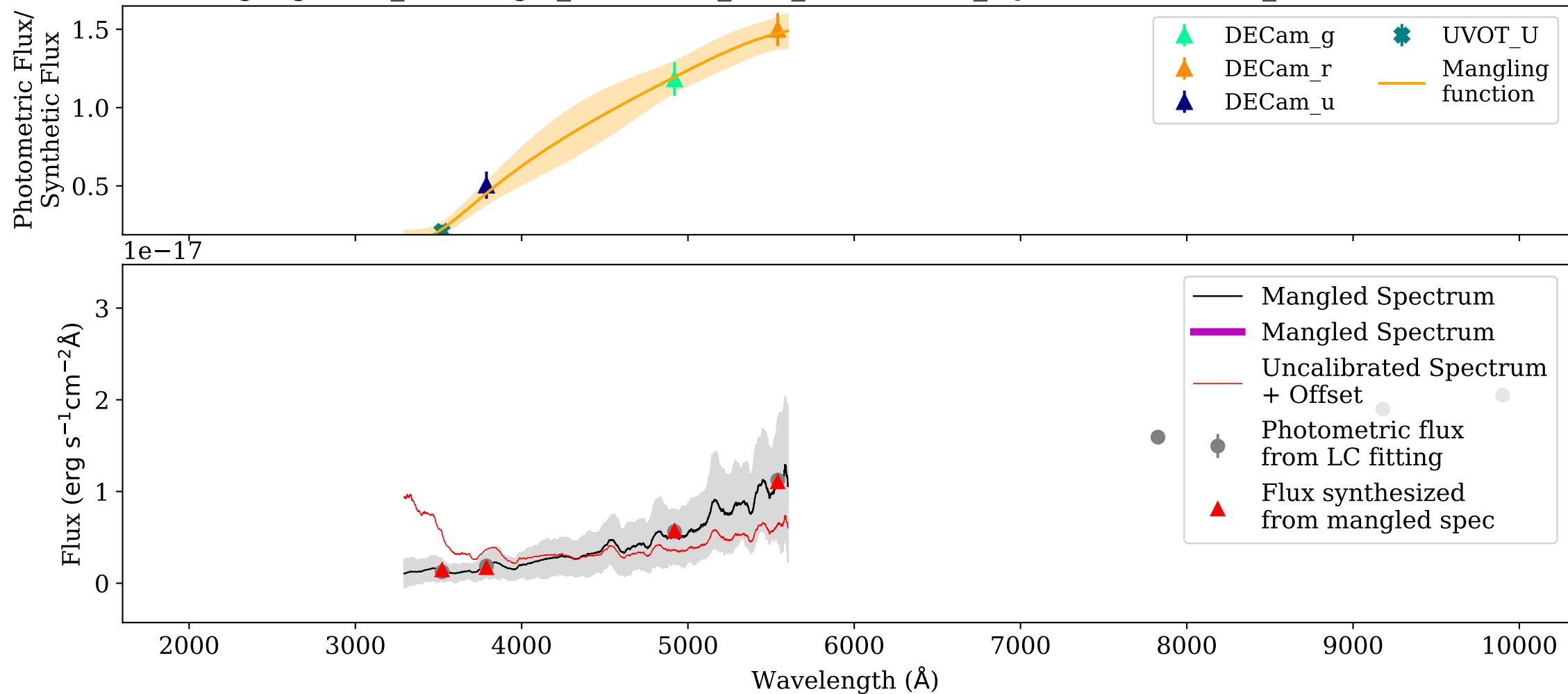
Mangling: UVB_AT2017gfo_ENGRAVE_v1.0_XSHOOTER_MJD-57990.000002_Phase+7.40d.dat
