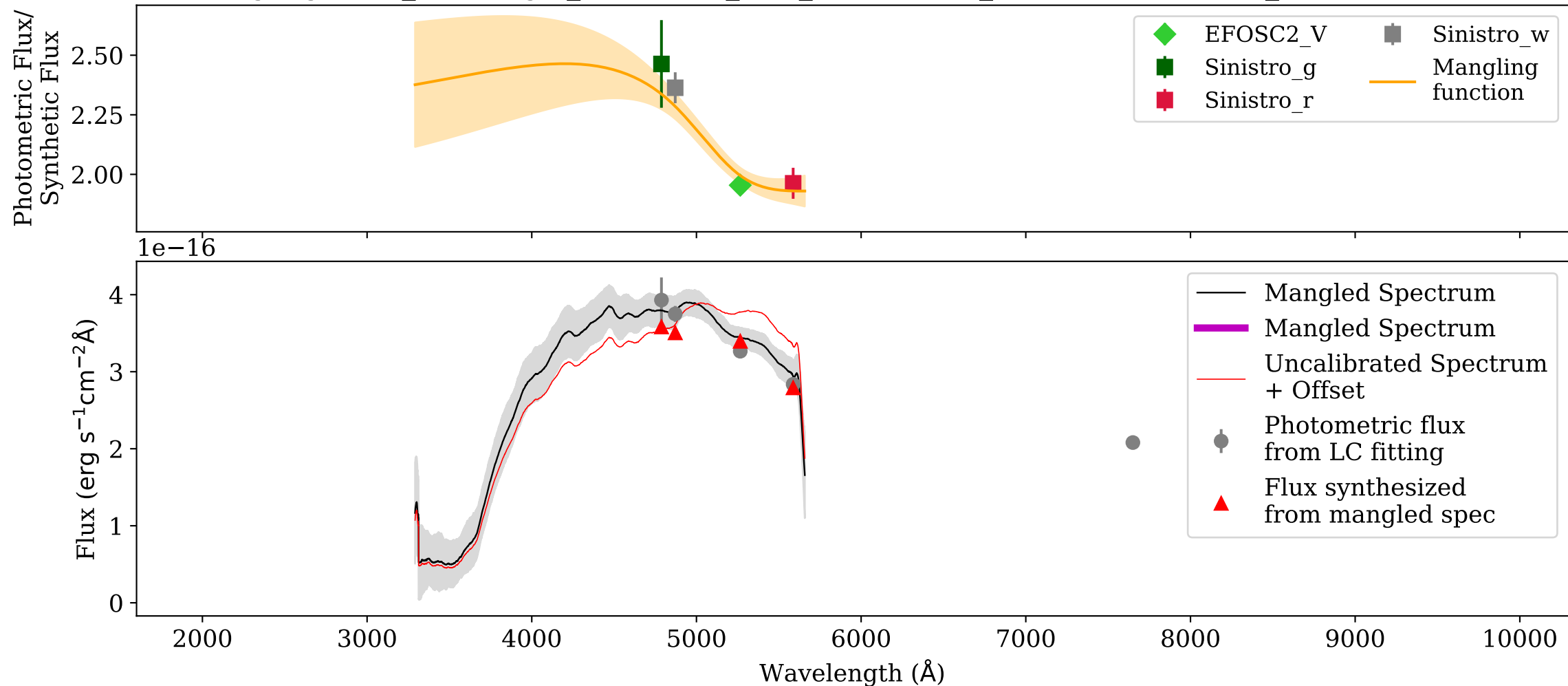
Mangling: UVB_AT2017gfo_ENGRAVE_v1.0_XSHOOTER_MJD-57983.969002_Phase+1.43d.dat
