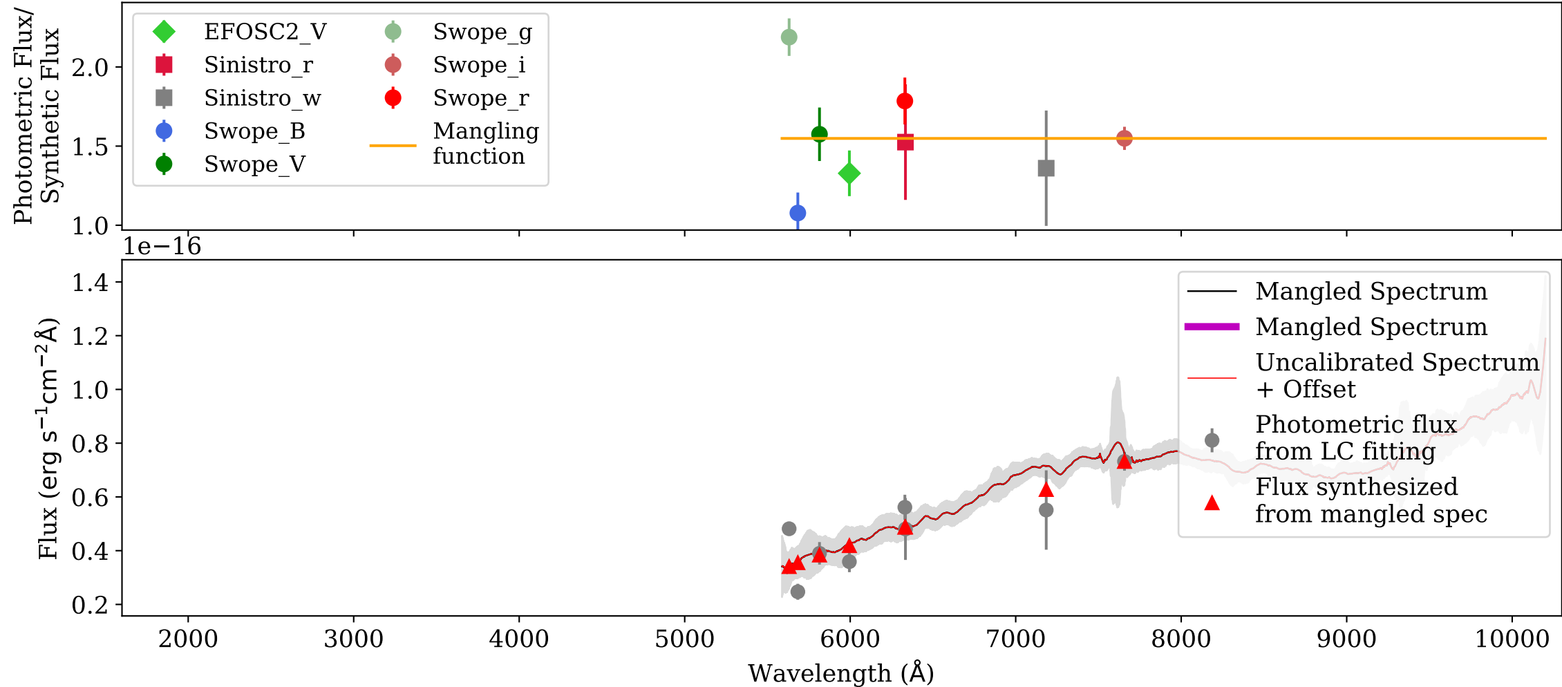
Mangling: VIS_AT2017gfo_ENGRAVE_v1.0_XSHOOTER_MJD-57985.974003_Phase+3.41d.dat
