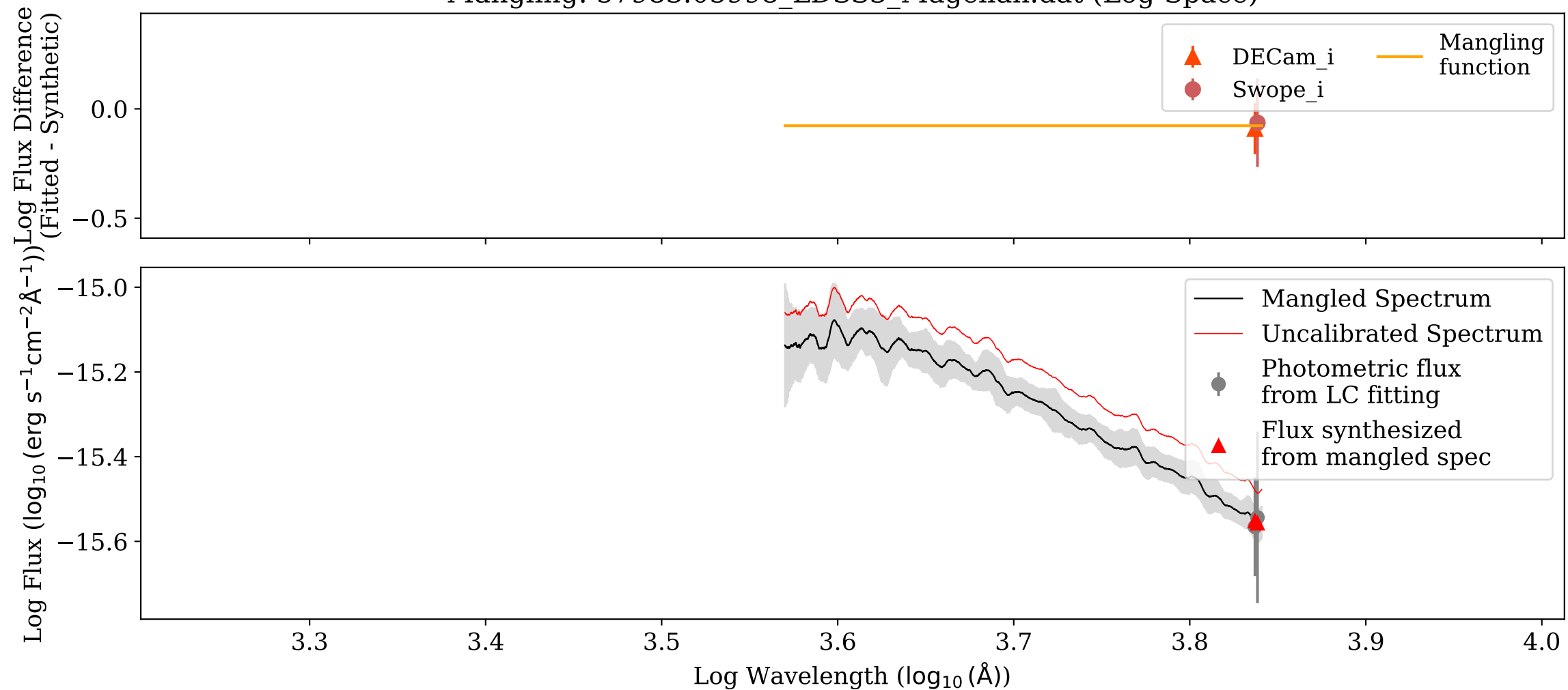
Mangling: 57983.05998_LDSS3_Magellan.dat (Log-Space)
