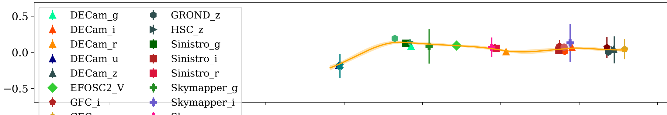
Mangling: 57983.9914_LDSS3_Magellan.dat (Log-Space)
