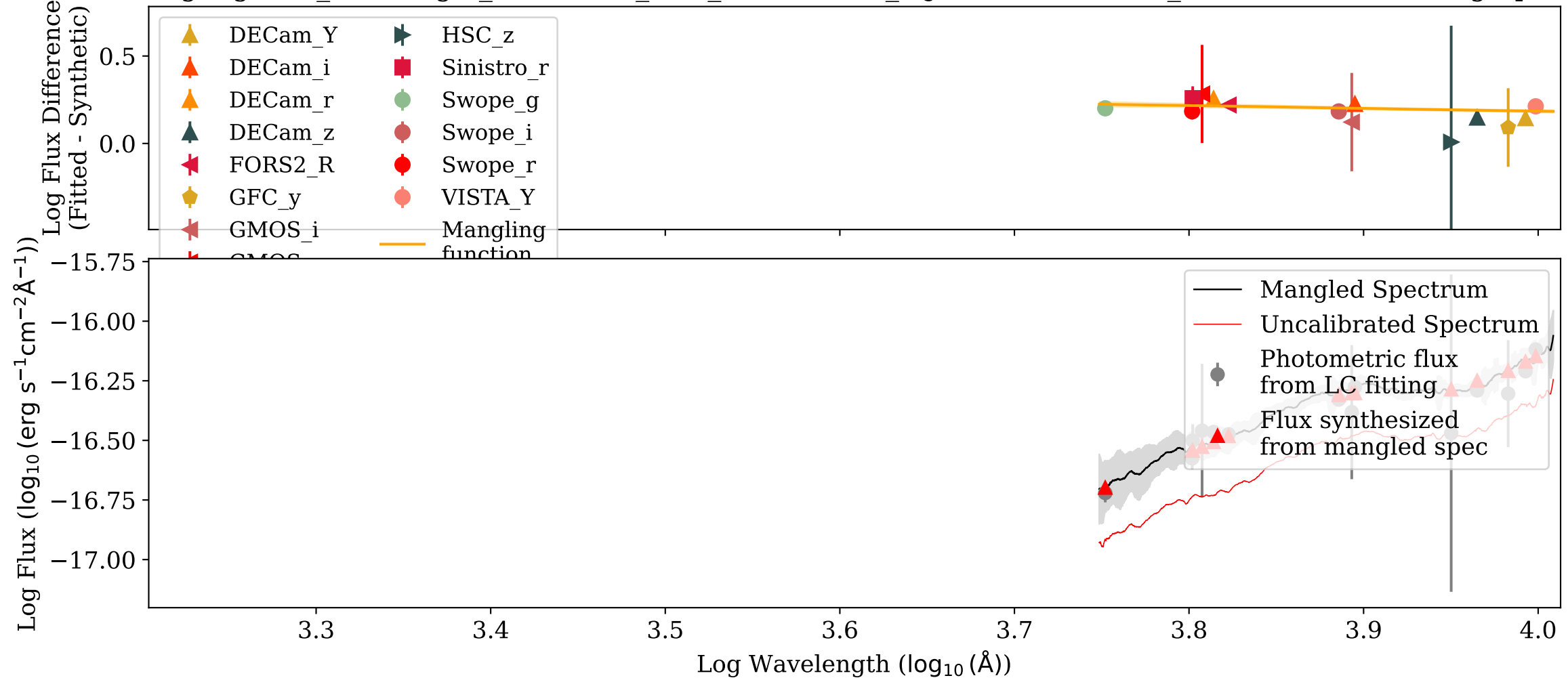
Mangling: VIS_AT2017gfo_ENGRAVE_v1.0_XSHOOTER_MJD-57986.974003_Phase+4.40d.dat (Log-Space)
