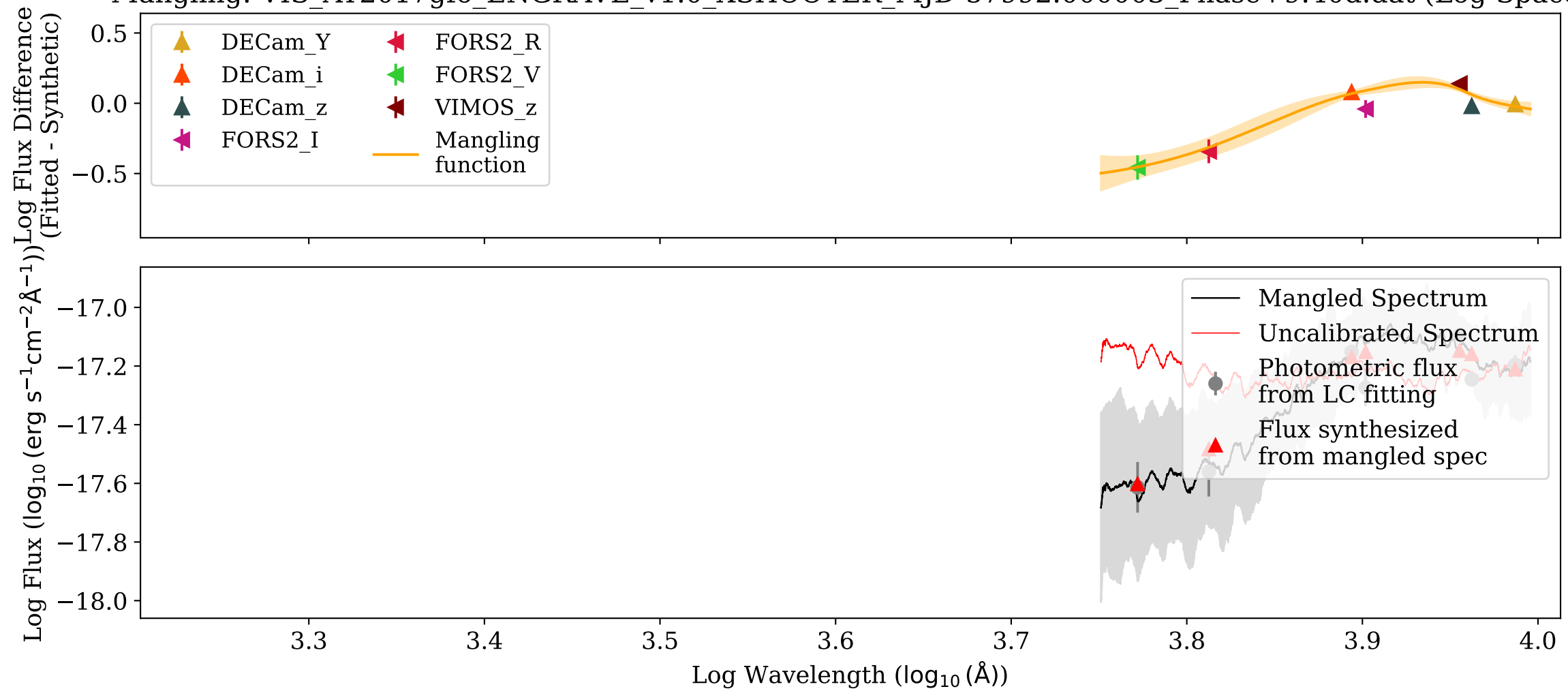
Mangling: VIS_AT2017gfo_ENGRAVE_v1.0_XSHOOTER_MJD-57992.000003_Phase+9.40d.dat (Log-Space)
