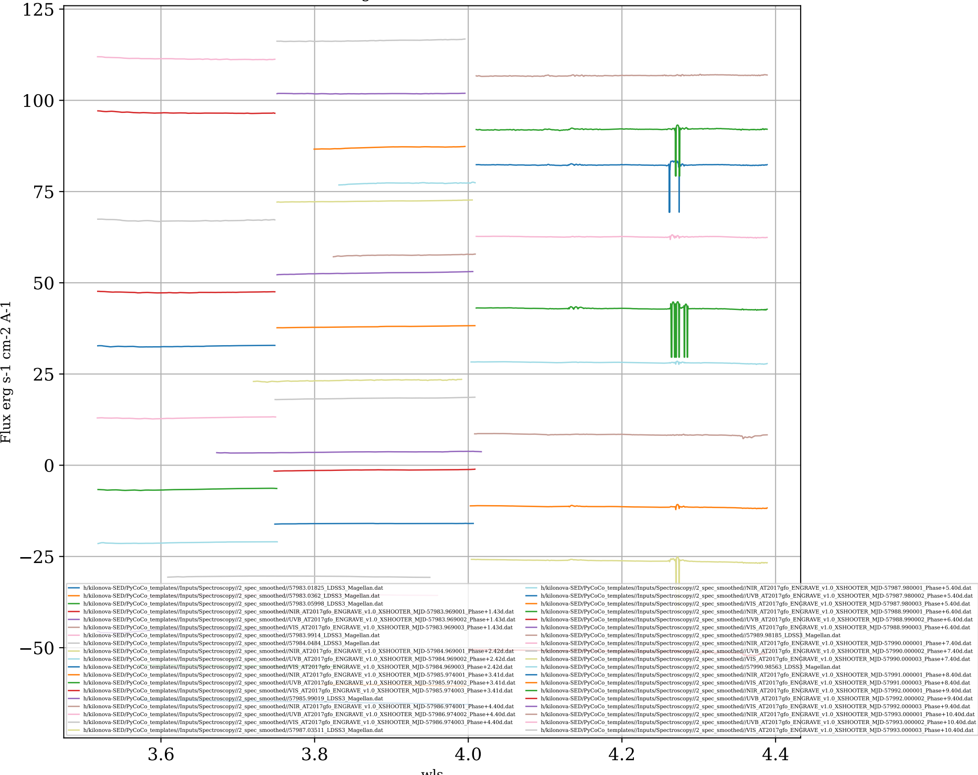
AT2017gfo MANGLED SPECTRA
