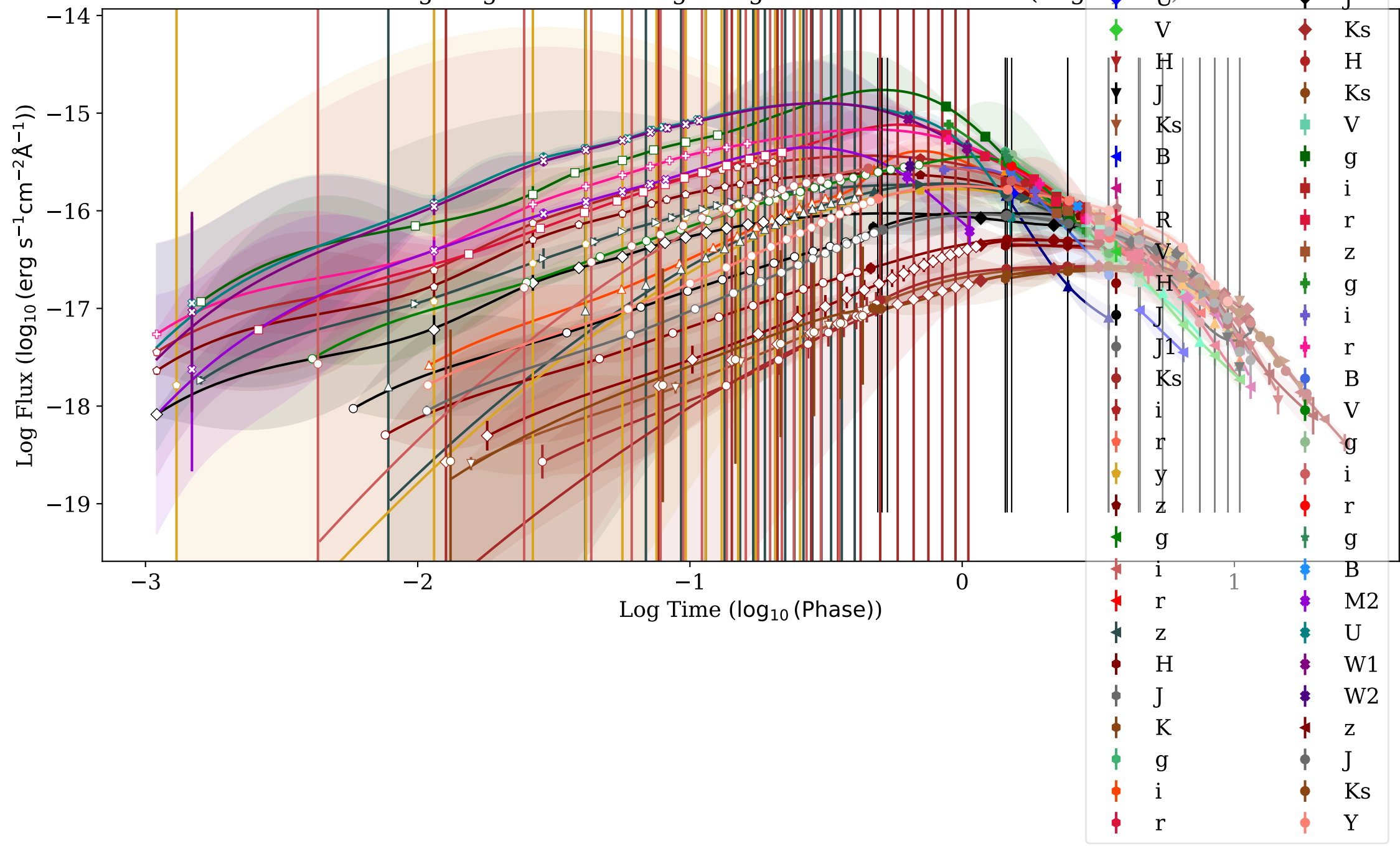
AT2017gfo light curve fitting using Gaussian Processes (Log-Space)
