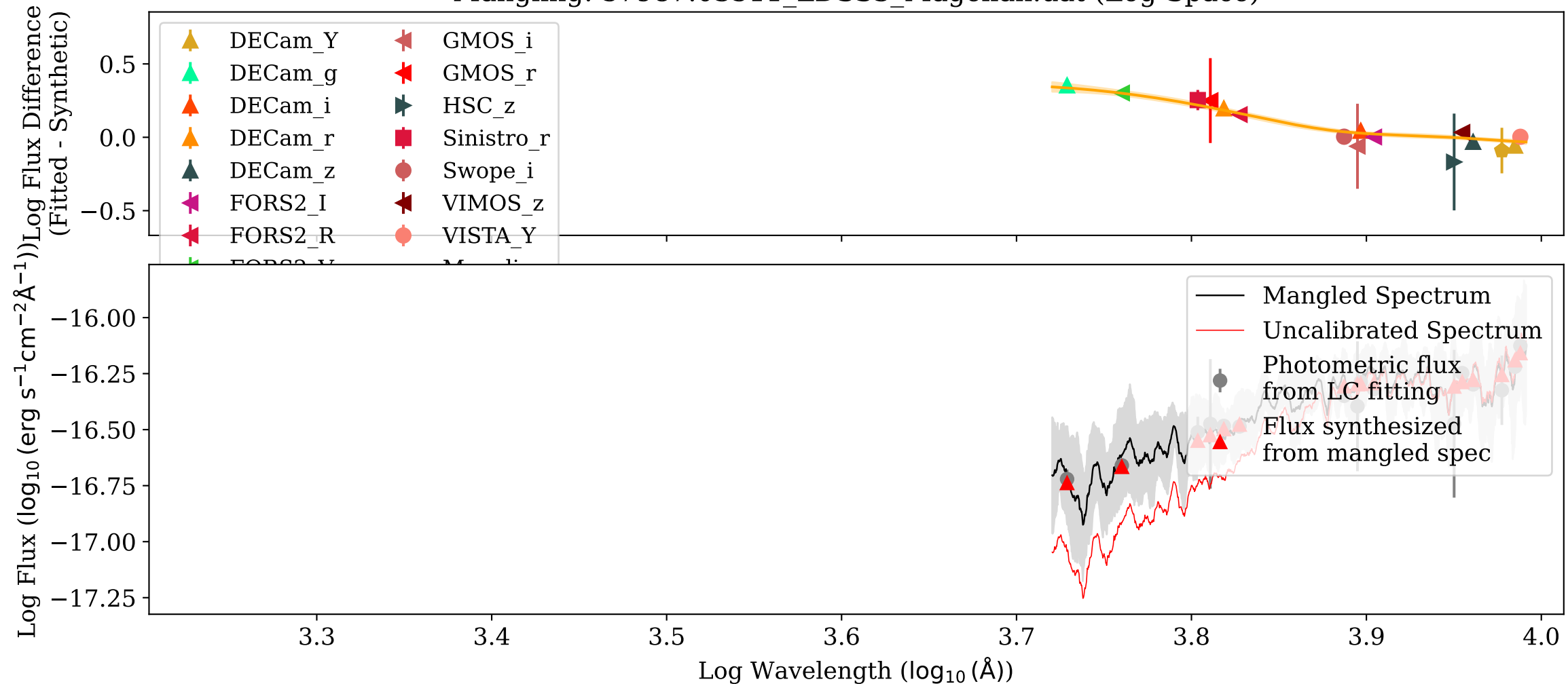
Mangling: 57987.03511_LDSS3_Magellan.dat (Log-Space)
