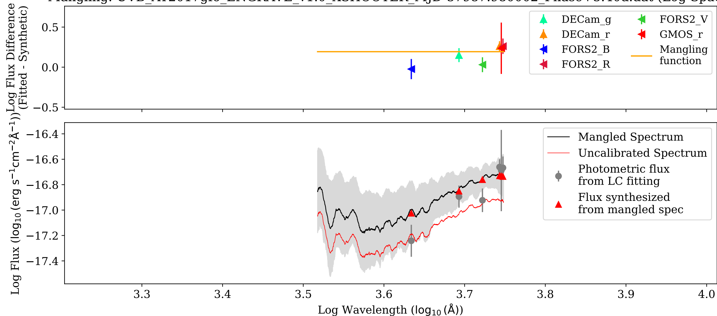
Mangling: UVB_AT2017gfo_ENGRAVE_v1.0_XSHOOTER_MJD-57987.980002_Phase+5.40d.dat (Log-Space)
