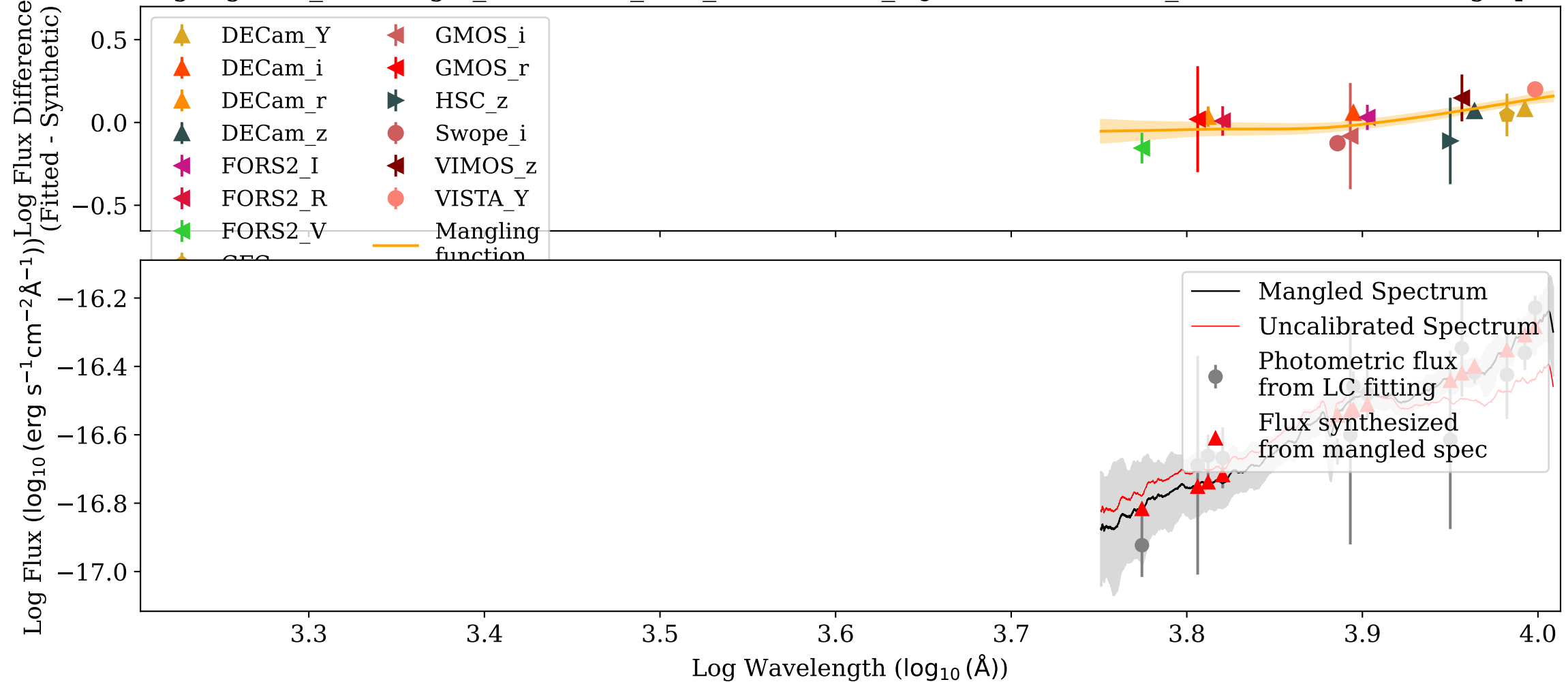
Mangling: VIS_AT2017gfo_ENGRAVE_v1.0_XSHOOTER_MJD-57987.980003_Phase+5.40d.dat (Log-Space)
