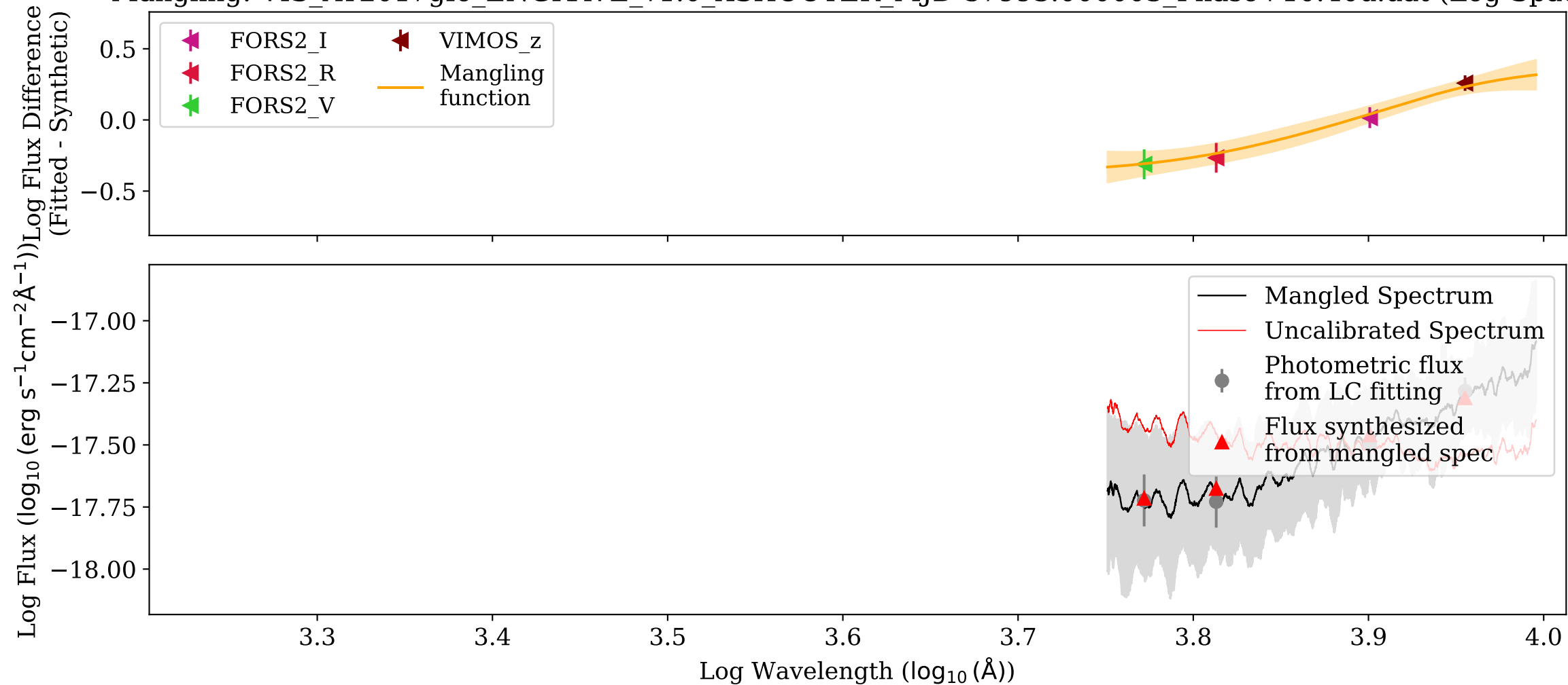
Mangling: VIS_AT2017gfo_ENGRAVE_v1.0_XSHOOTER_MJD-57993.000003_Phase+10.40d.dat (Log-Space)
