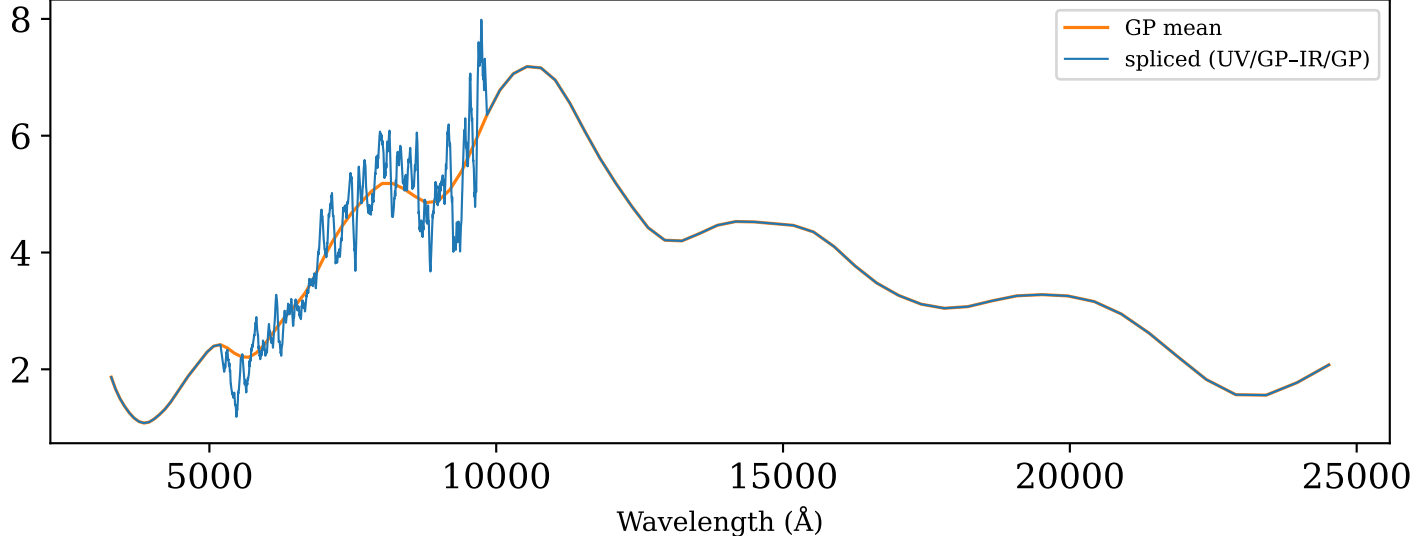
AT2017gfo log10 phase=0.653898
