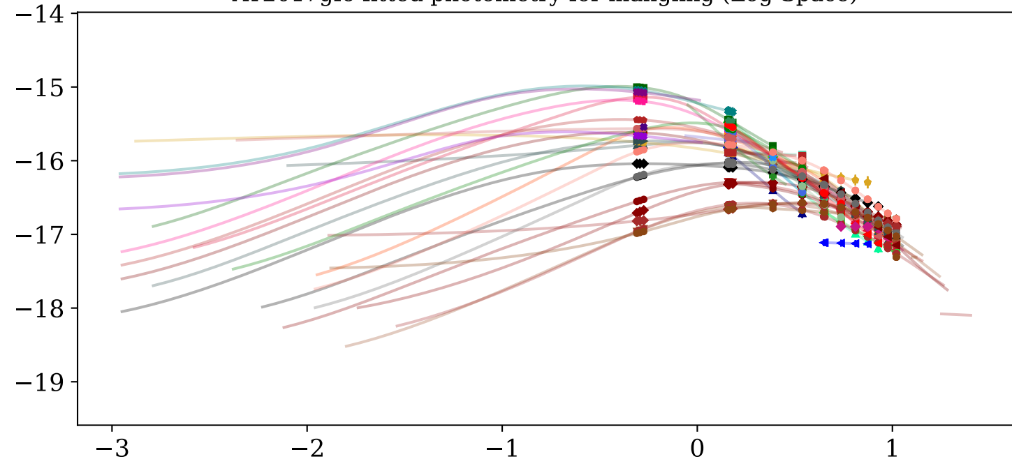
AT2017gfo fitted photometry for mangling (Log-Space)
