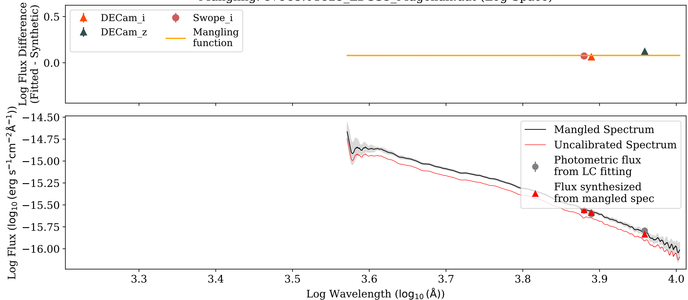
Mangling: 57983.01825_LDSS3_Magellan.dat (Log-Space)
