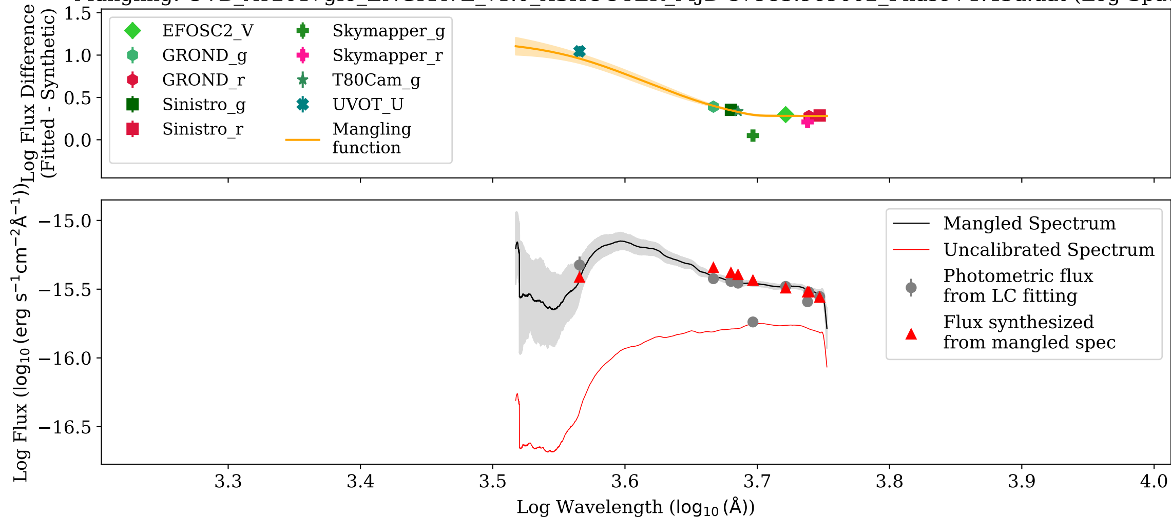
Mangling: UVB_AT2017gfo_ENGRAVE_v1.0_XSHOOTER_MJD-57983.969002_Phase+1.43d.dat (Log-Space)
