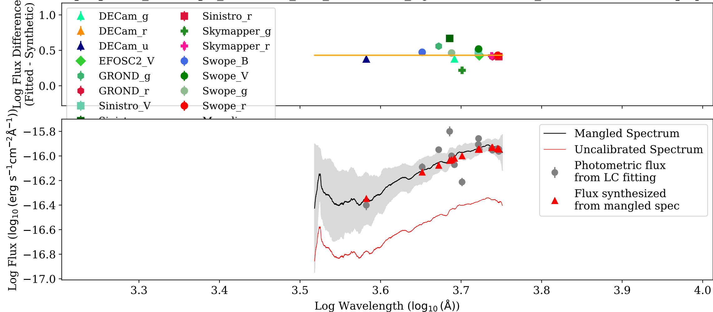
Mangling: UVB_AT2017gfo_ENGRAVE_v1.0_XSHOOTER_MJD-57984.969002_Phase+2.42d.dat (Log-Space)
