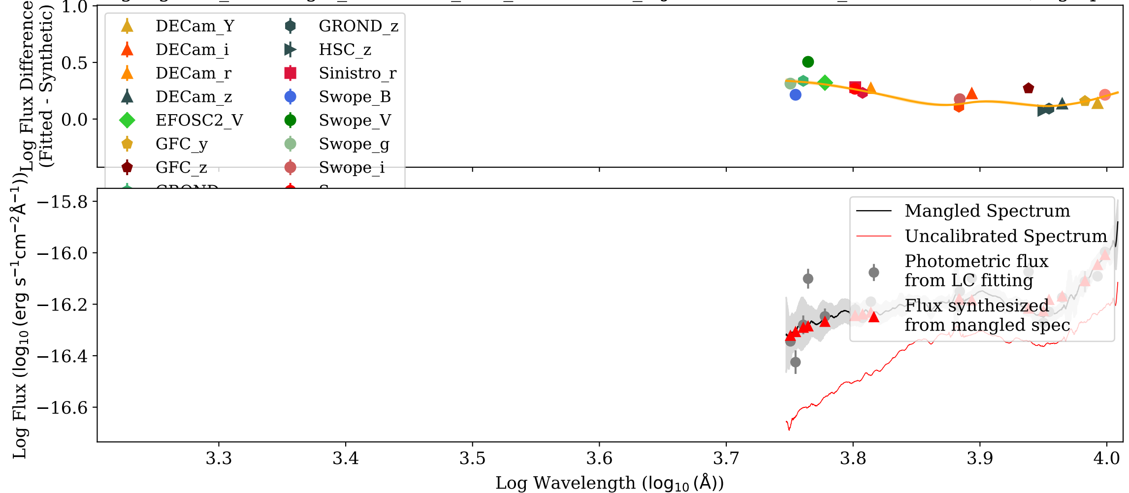
Mangling: VIS_AT2017gfo_ENGRAVE_v1.0_XSHOOTER_MJD-57985.974003_Phase+3.41d.dat (Log-Space)
