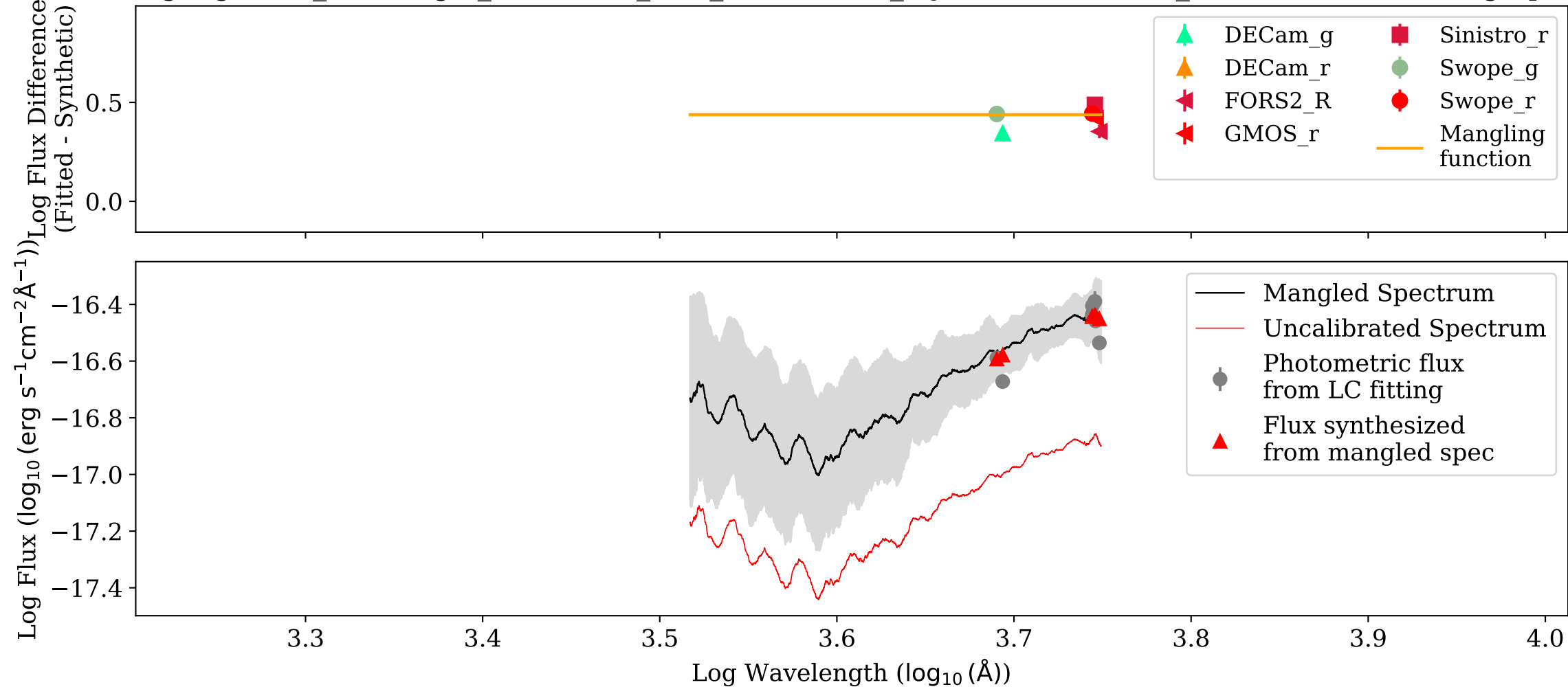
Mangling: UVB_AT2017gfo_ENGRAVE_v1.0_XSHOOTER_MJD-57986.974002_Phase+4.40d.dat (Log-Space)
