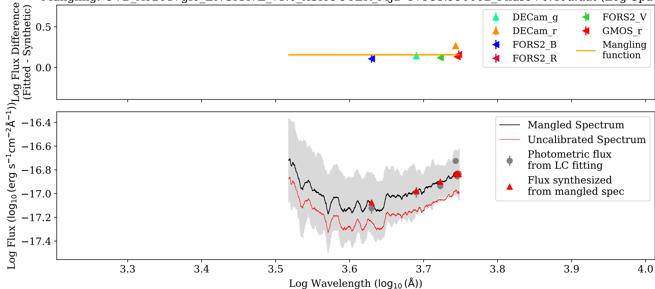
Mangling: UVB_AT2017gfo_ENGRAVE_v1.0_XSHOOTER_MJD-57988.990002_Phase+6.40d.dat (Log-Space)
