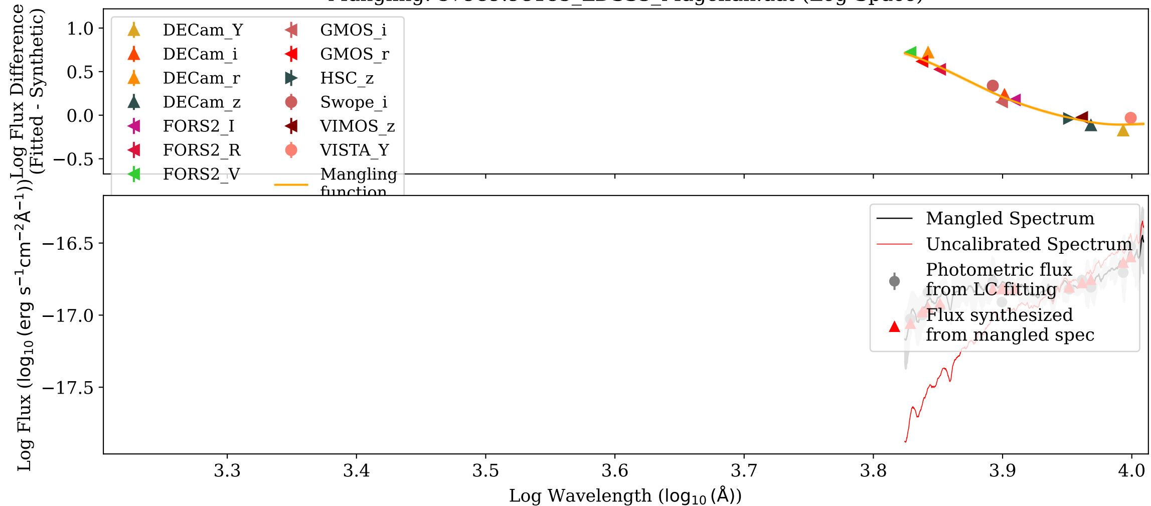
Mangling: 57989.98185_LDSS3_Magellan.dat (Log-Space)
