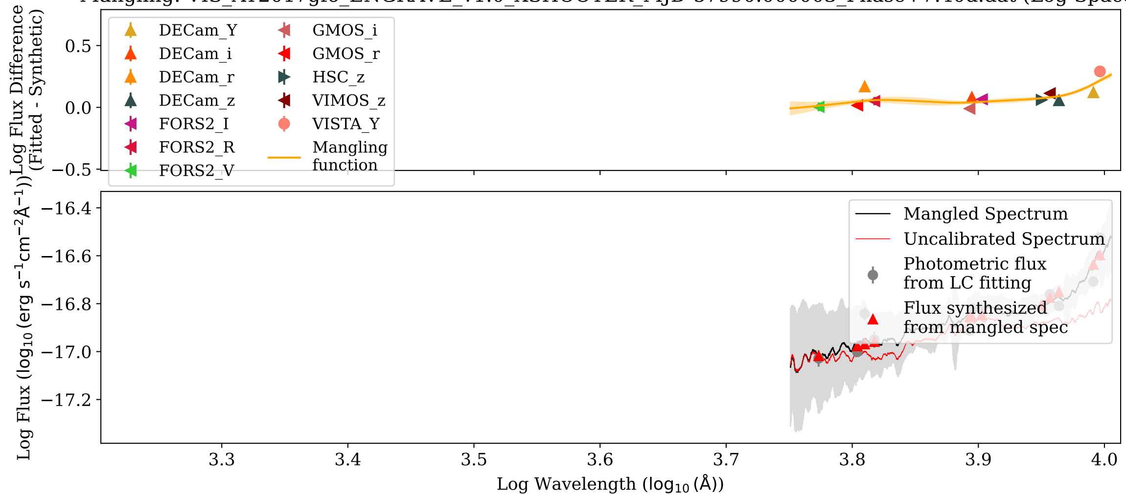
Mangling: VIS_AT2017gfo_ENGRAVE_v1.0_XSHOOTER_MJD-57990.000003_Phase+7.40d.dat (Log-Space)
