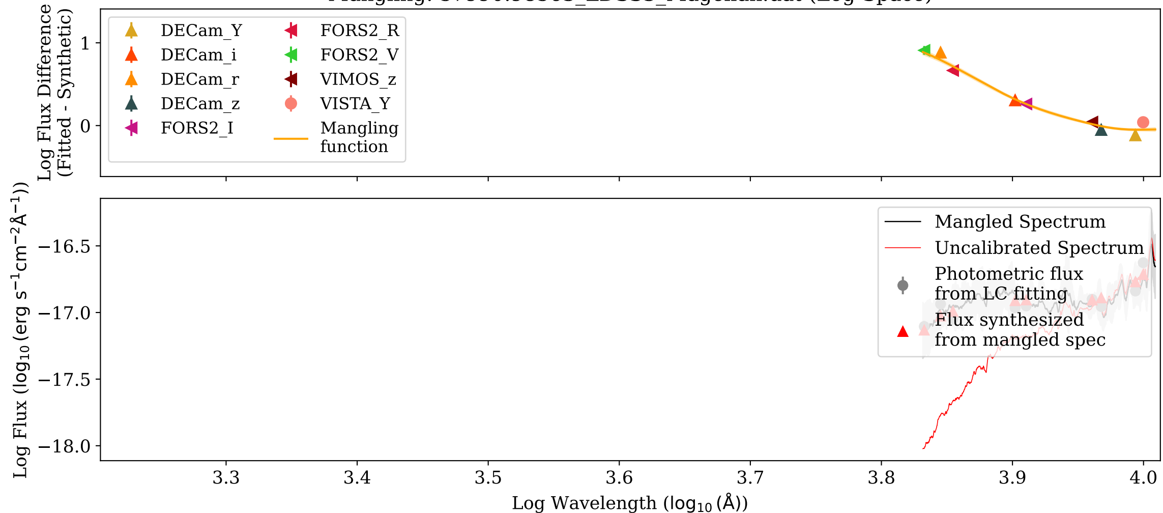
Mangling: 57990.98563_LDSS3_Magellan.dat (Log-Space)
