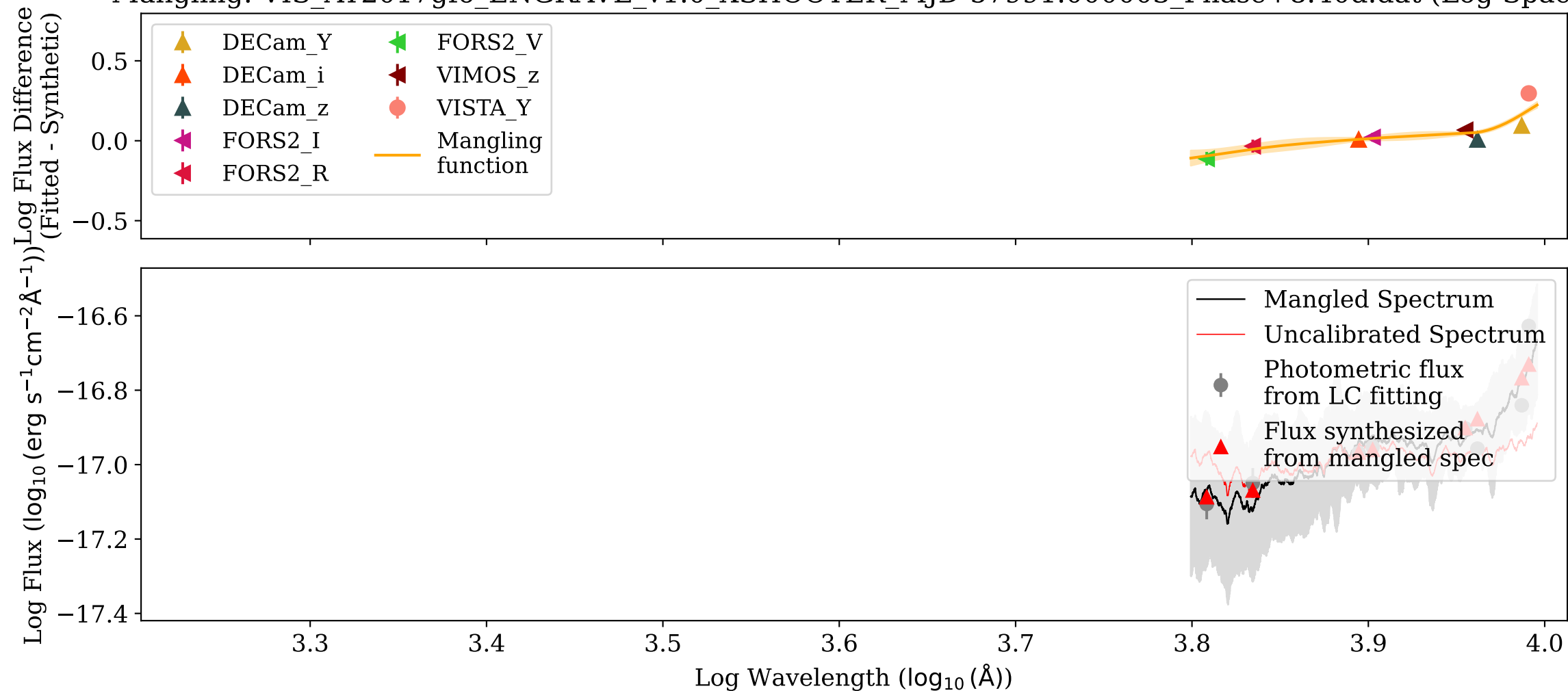
Mangling: VIS_AT2017gfo_ENGRAVE_v1.0_XSHOOTER_MJD-57991.000003_Phase+8.40d.dat (Log-Space)
