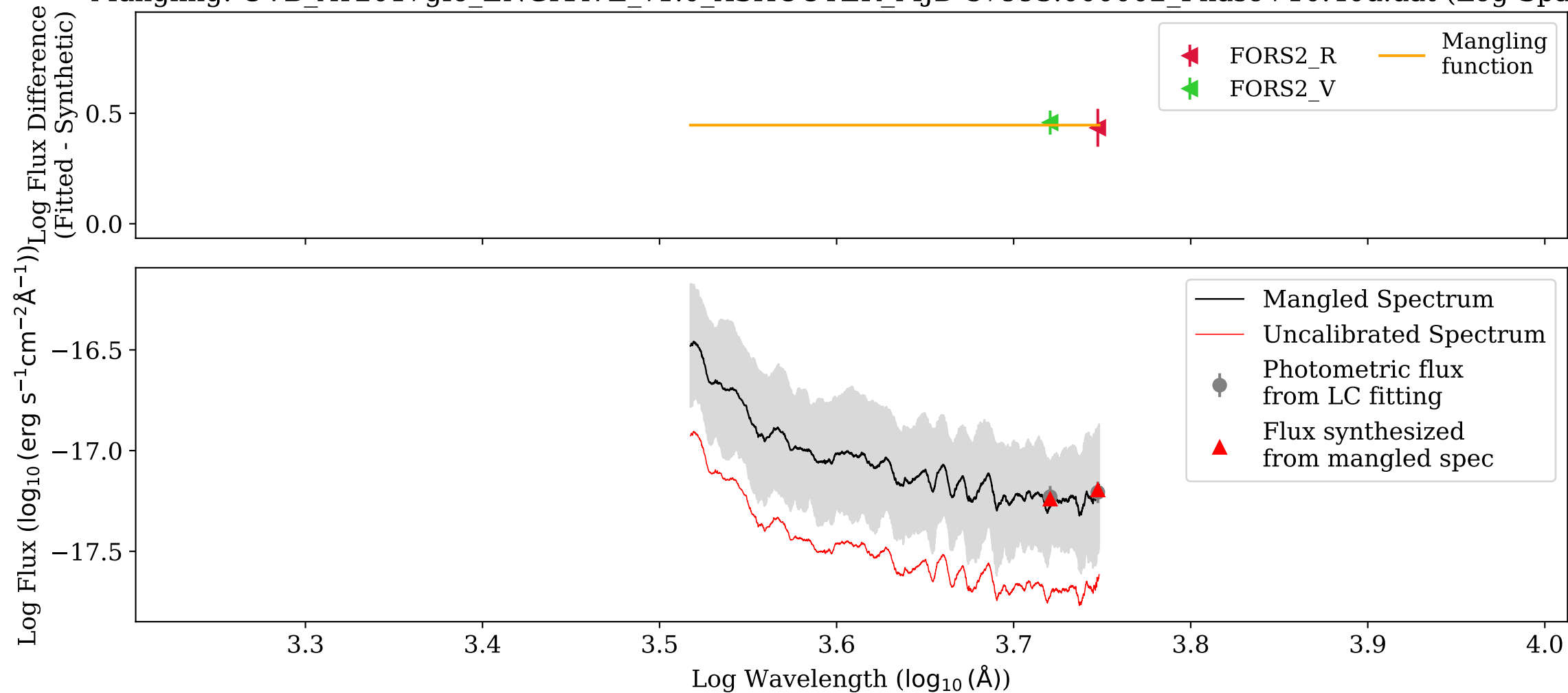
Mangling: UVB_AT2017gfo_ENGRAVE_v1.0_XSHOOTER_MJD-57993.000002_Phase+10.40d.dat (Log-Space)
