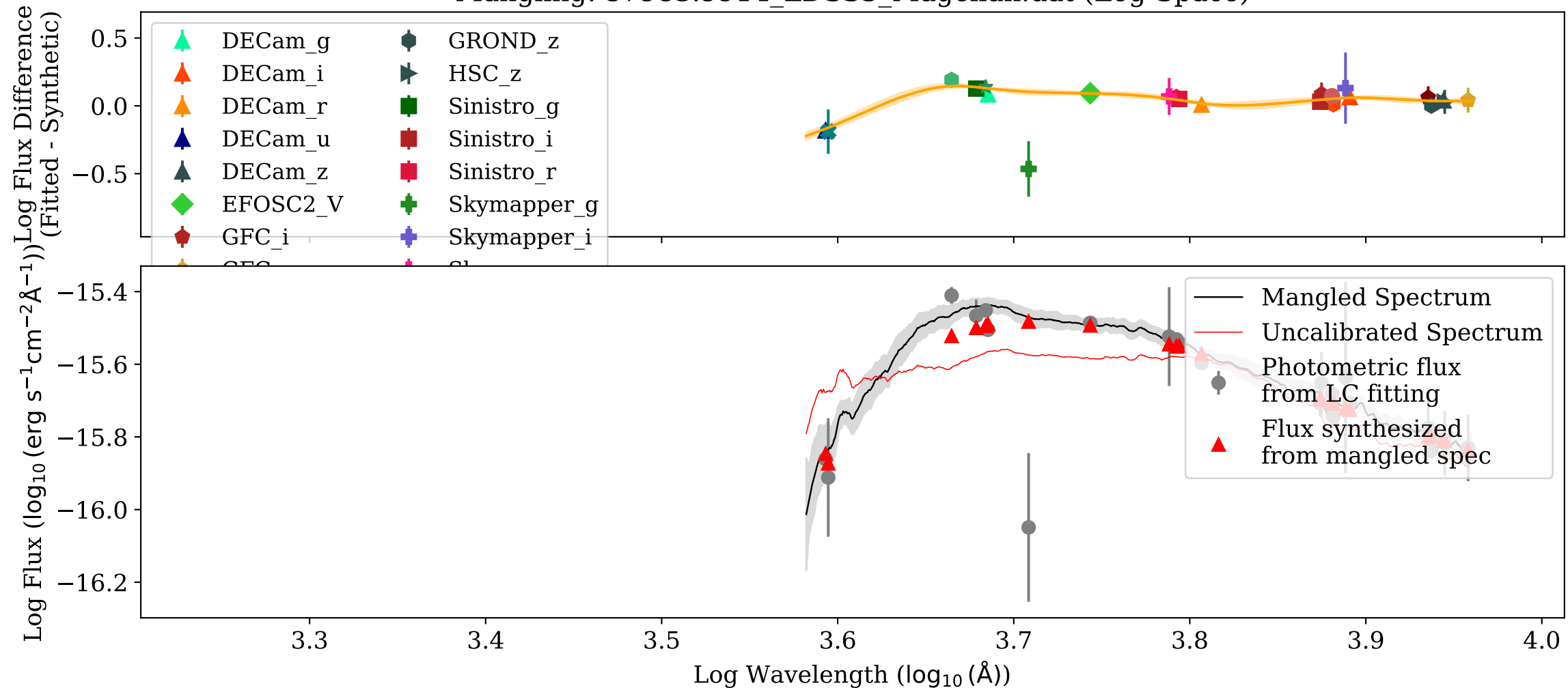
Mangling: 57983.9914_LDSS3_Magellan.dat (Log-Space)
