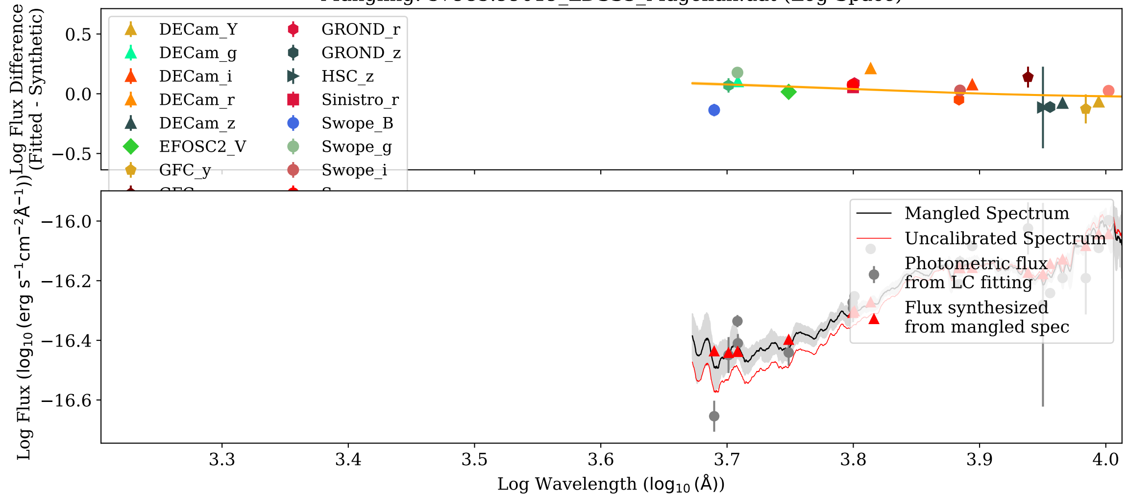
Mangling: 57985.99019_LDSS3_Magellan.dat (Log-Space)
