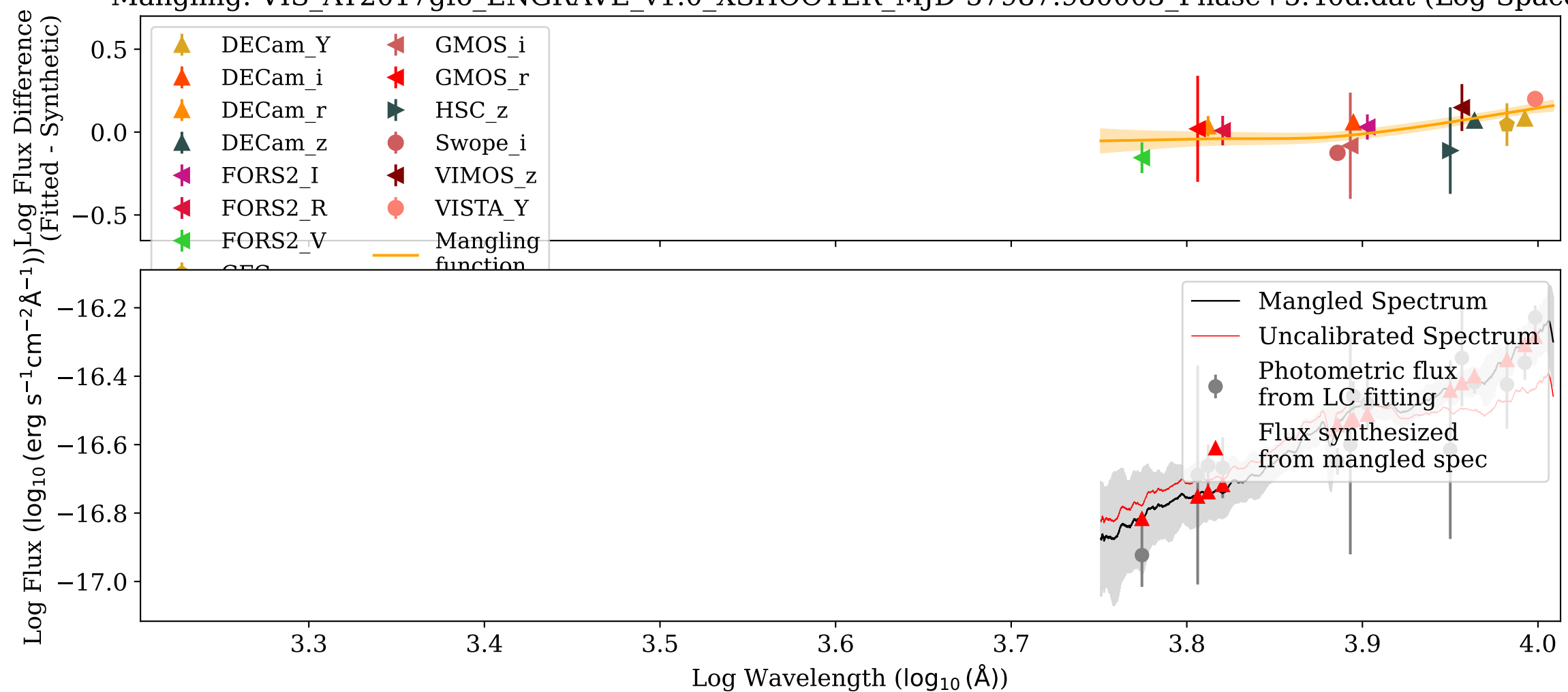
Mangling: VIS_AT2017gfo_ENGRAVE_v1.0_XSHOOTER_MJD-57987.980003_Phase+5.40d.dat (Log-Space)
