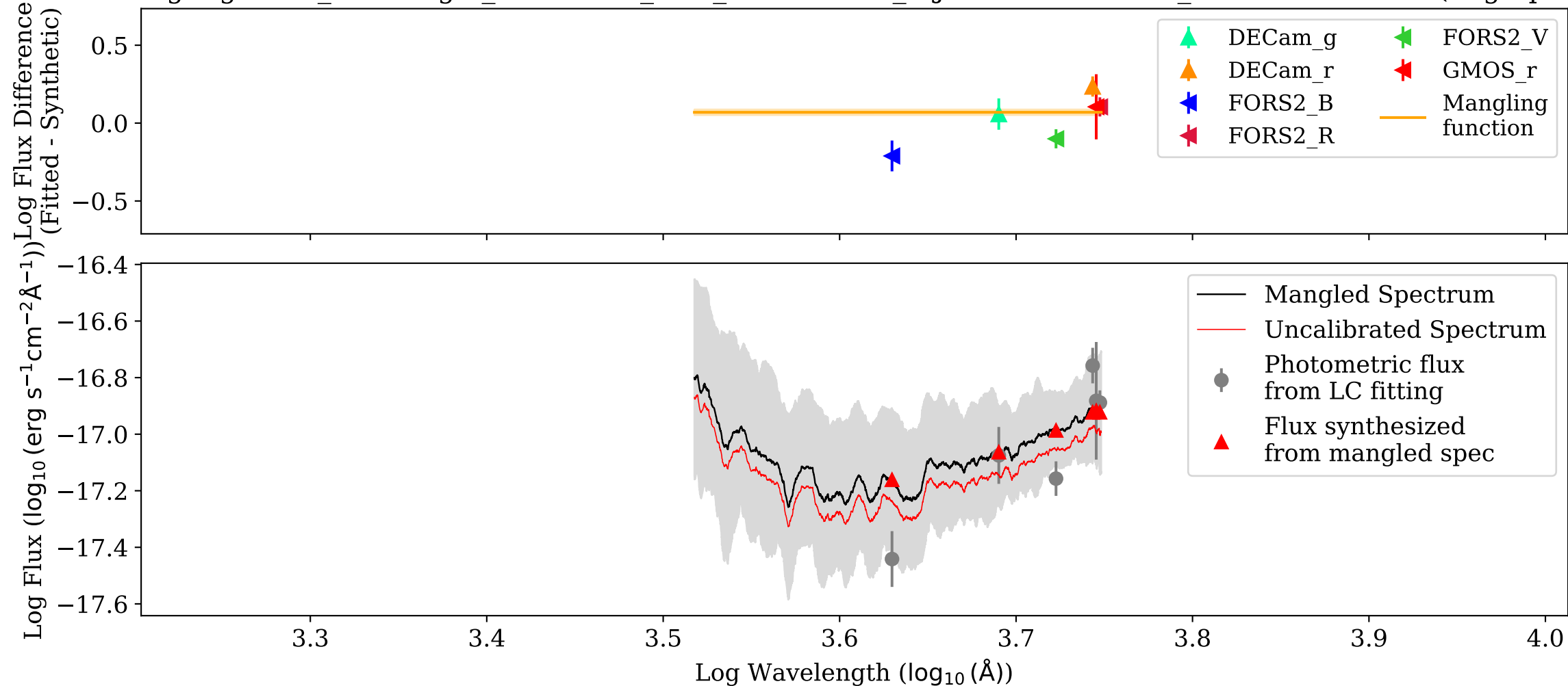
Mangling: UVB_AT2017gfo_ENGRAVE_v1.0_XSHOOTER_MJD-57988.990002_Phase+6.40d.dat (Log-Space)
