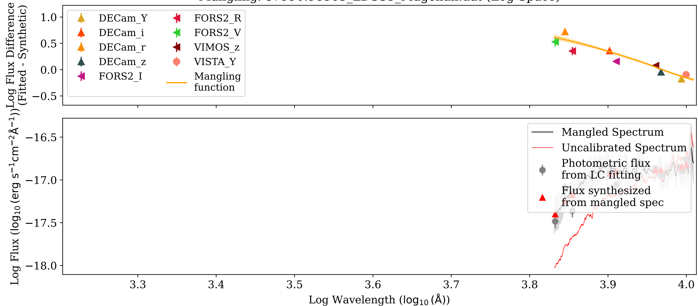
Mangling: 57990.98563_LDSS3_Magellan.dat (Log-Space)
