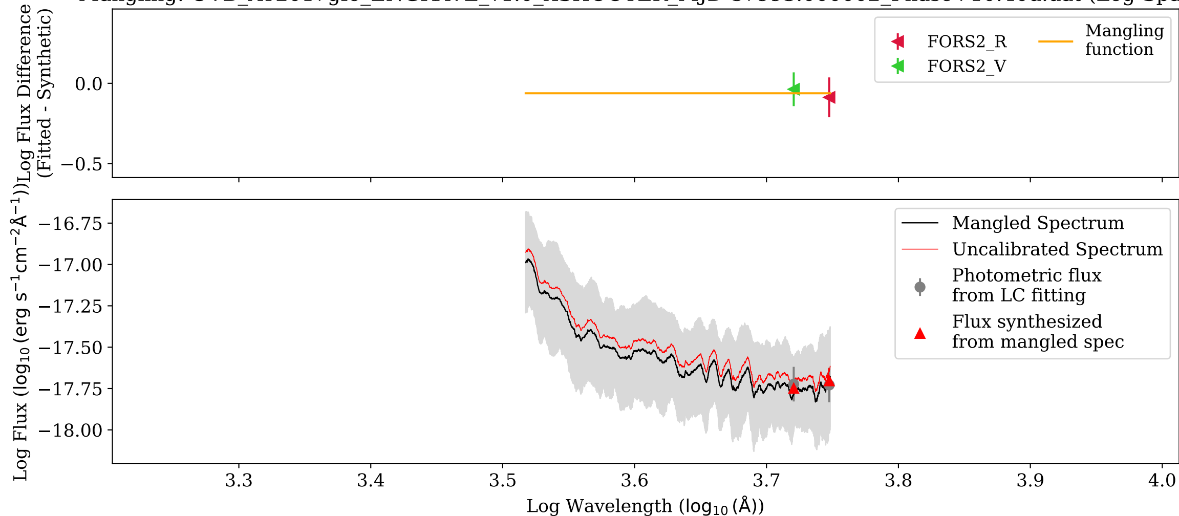
Mangling: UVB_AT2017gfo_ENGRAVE_v1.0_XSHOOTER_MJD-57993.000002_Phase+10.40d.dat (Log-Space)
