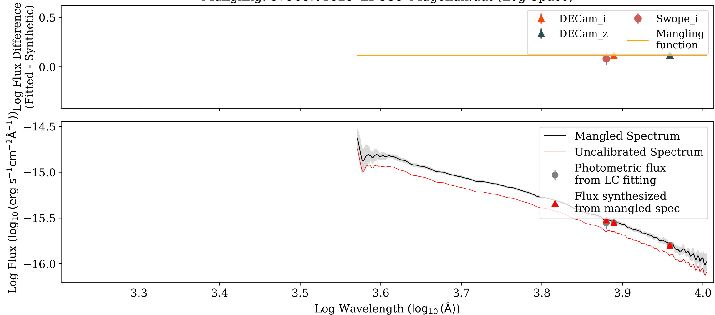
Mangling: 57983.01825_LDSS3_Magellan.dat (Log-Space)
