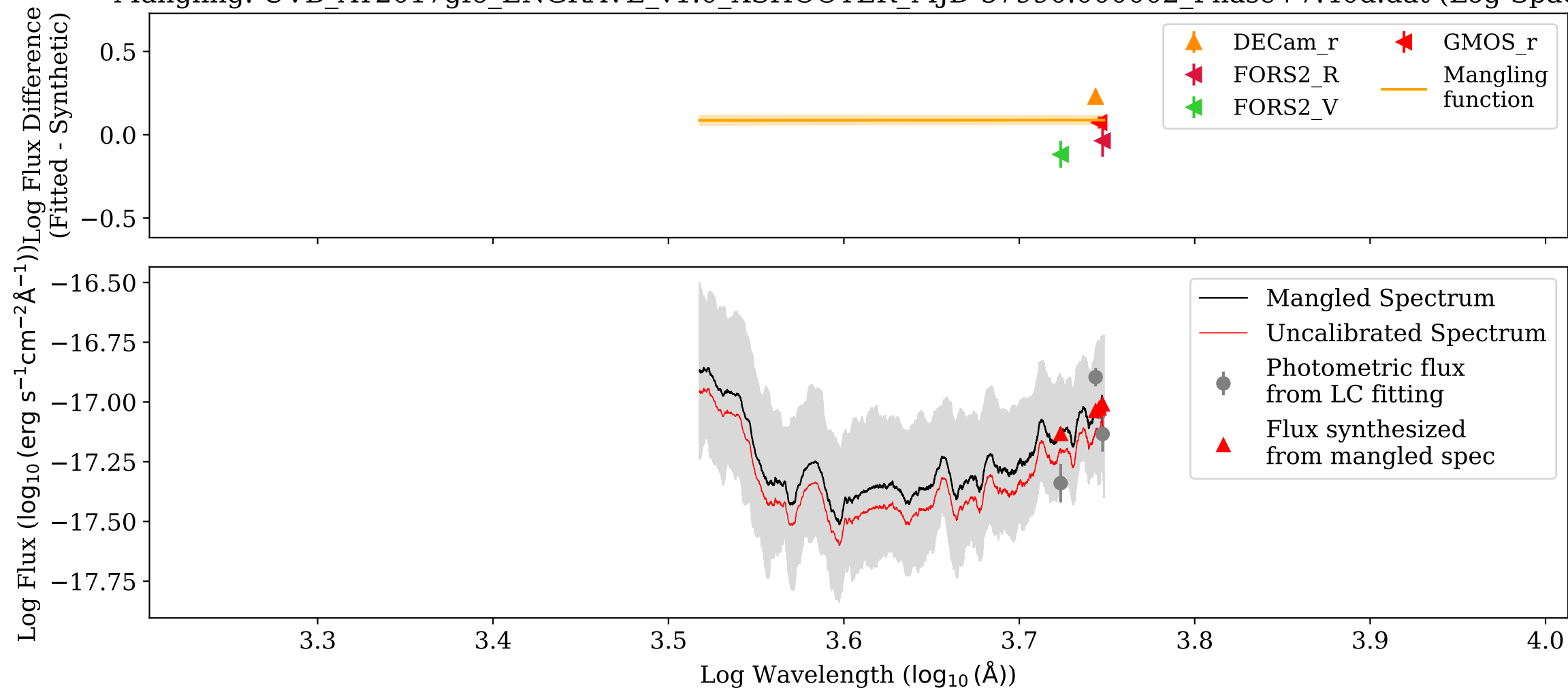
Mangling: UVB_AT2017gfo_ENGRAVE_v1.0_XSHOOTER_MJD-57990.000002_Phase+7.40d.dat (Log-Space)
