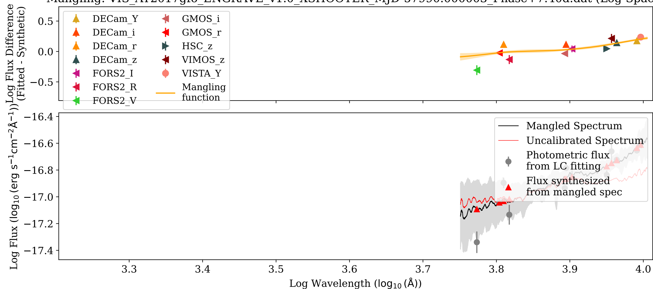
Mangling: VIS_AT2017gfo_ENGRAVE_v1.0_XSHOOTER_MJD-57990.000003_Phase+7.40d.dat (Log-Space)
