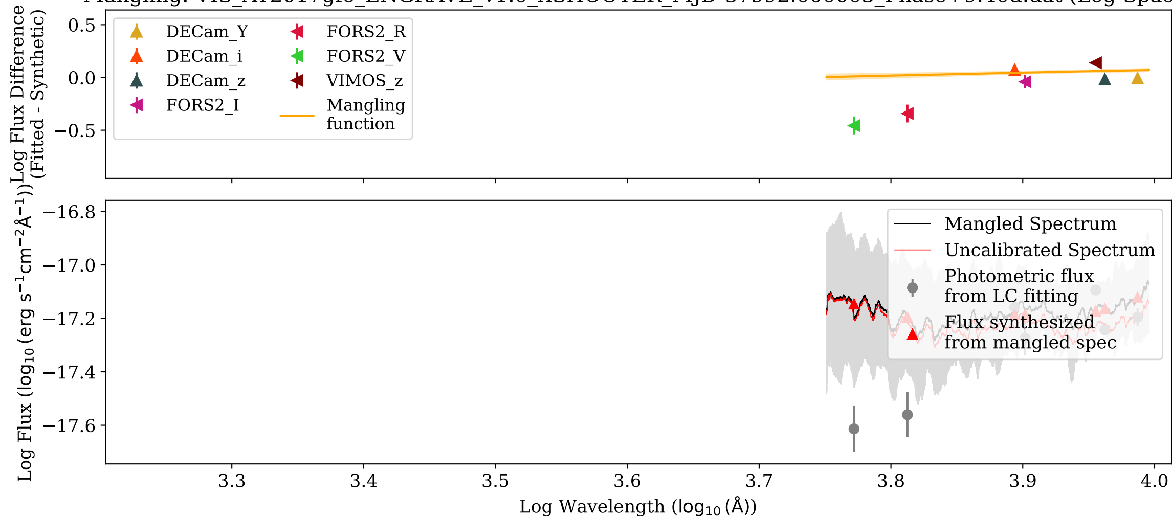
Mangling: VIS_AT2017gfo_ENGRAVE_v1.0_XSHOOTER_MJD-57992.000003_Phase+9.40d.dat (Log-Space)
