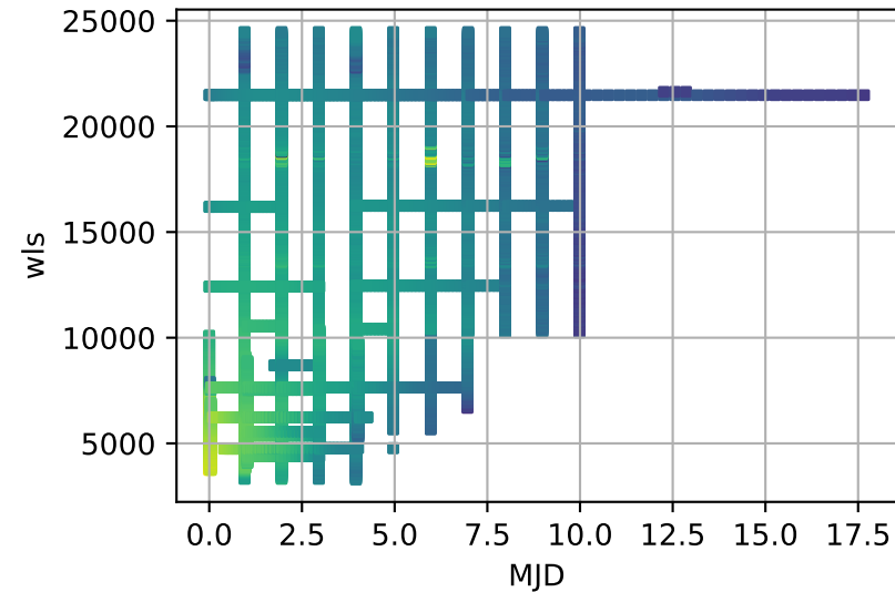
Training Data
