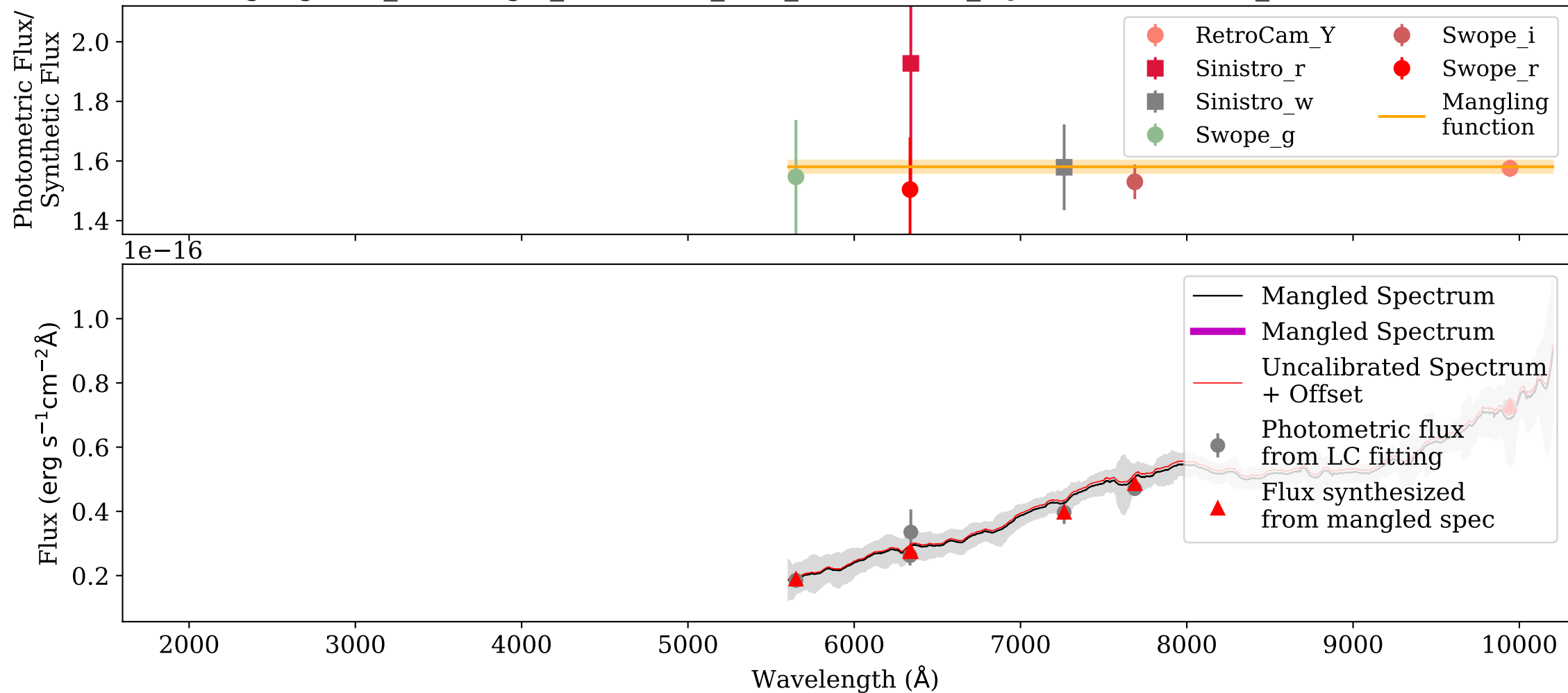
Mangling: VIS_AT2017gfo_ENGRAVE_v1.0_XSHOOTER_MJD-57986.974003_Phase+4.40d.dat
