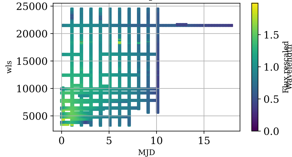
Training Data
