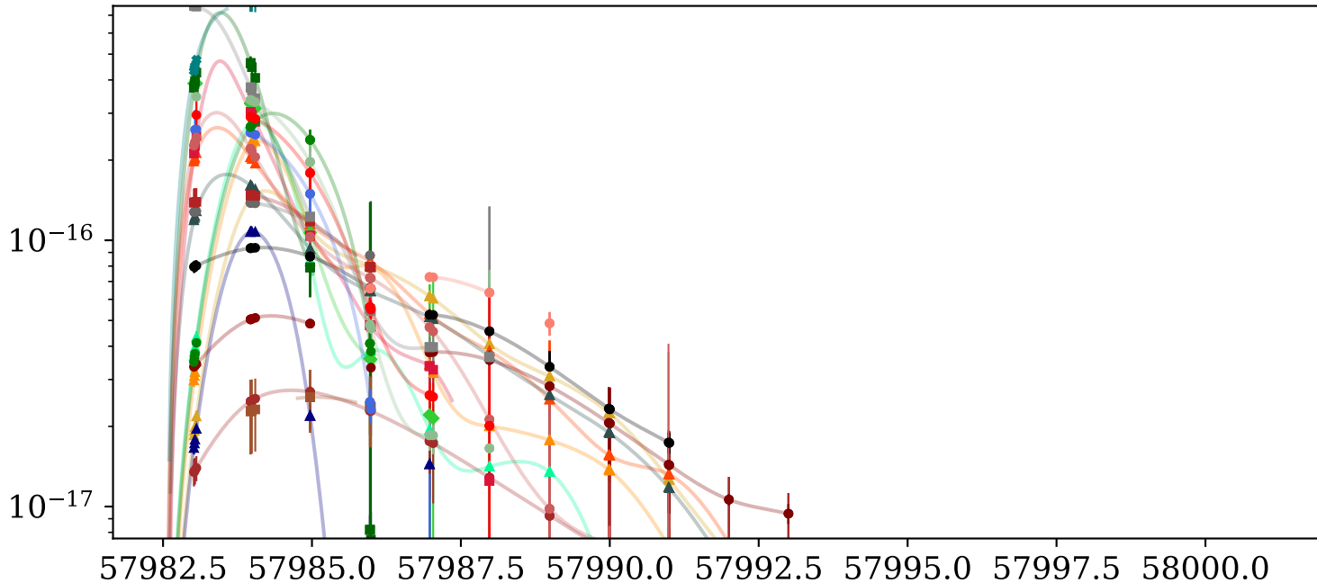
AT2017gfo fitted photometry for mangling
