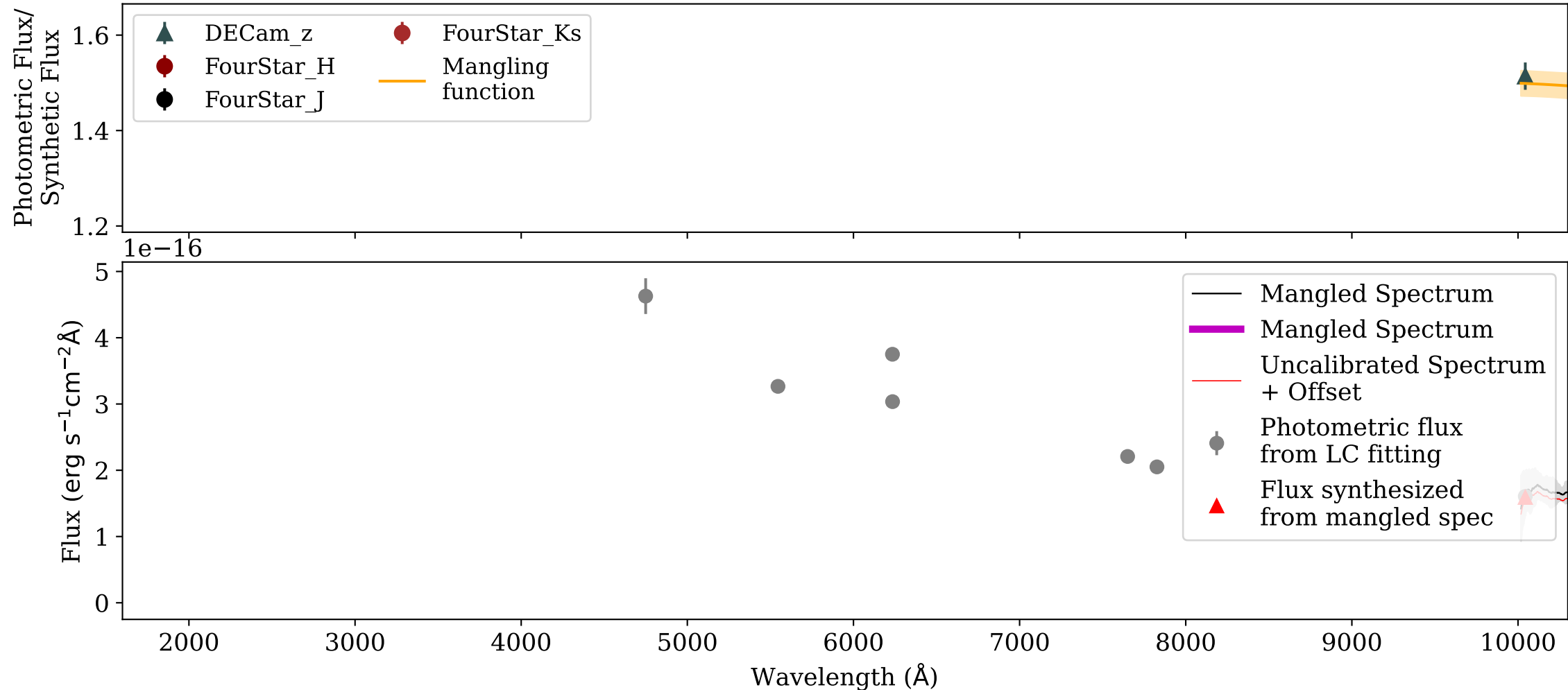
Mangling: NIR_AT2017gfo_ENGRAVE_v1.0_XSHOOTER_MJD-57983.969001_Phase+1.43d.dat
