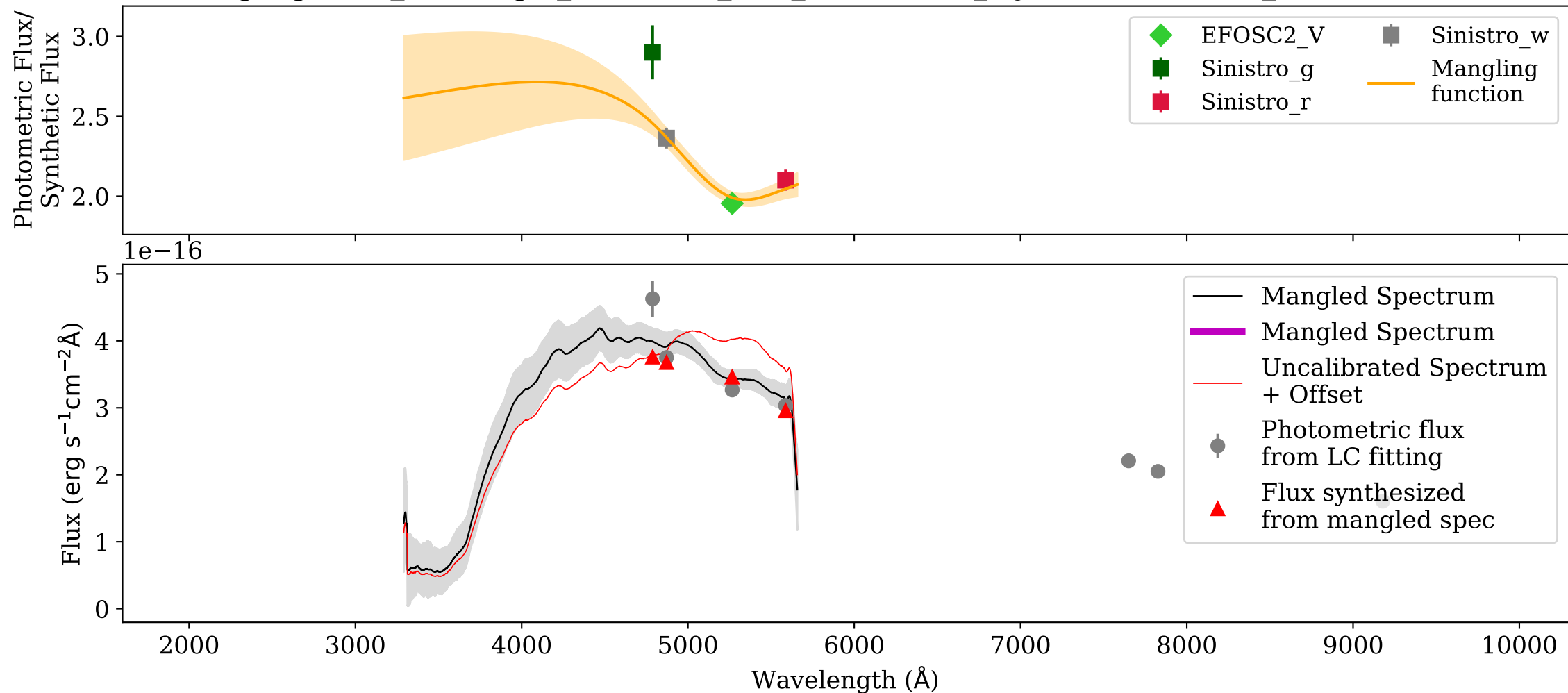
Mangling: UVB_AT2017gfo_ENGRAVE_v1.0_XSHOOTER_MJD-57983.969002_Phase+1.43d.dat
